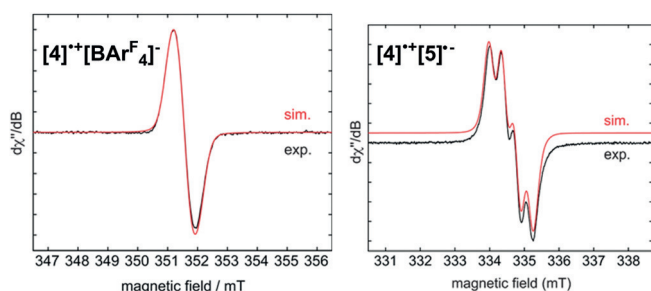
Figure 4. Experimental (black) and simulated (red) EPR spectra of [4]^+[\text{BARF}_4]^- in o -difluorobenzene (left) and [4]^+[\text{5}]^- in hexanes (right) at room temperature. Simulated parameters are as follows: [4]^+[\text{BARF}_4]^- g_{\text{iso}} = 2.0023 , a(\text{B}) = \text{ca. } 1.7 \text{ G} (peak-to-peak width = 7 G), [4]^+[\text{5}]^- g_{\text{iso}} = 2.0025 , a(\text{B}) = 3.5 \text{ G} ( [\text{5}]^- ); g_{\text{iso}} = 2.0023 , a(\text{B}) < 1 \text{ G} ( [4]^+ ).
