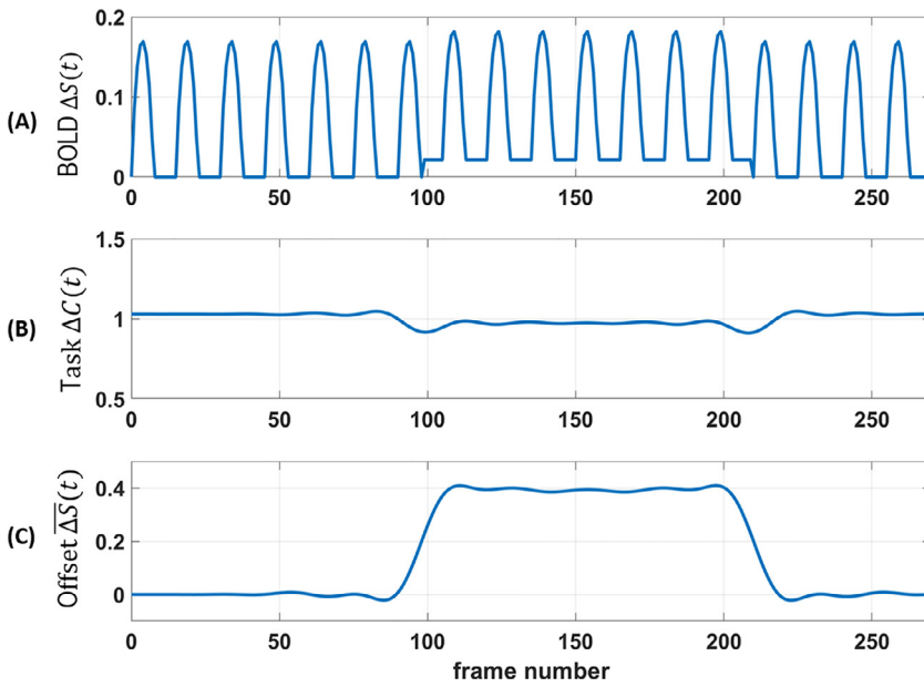
Fig. 1. Simulation. (A) Model of BOLD contrast during task with half-sinusoidal CMRO 2 variation, square wave increases in CBF during time frames 100-210, A=0.02 . Simulation set maximum BOLD factor M=1 . (B) Sliding window analysis of task contrast (Eq. 4b) does not vary substantially during elevated CBF (except artifactually at transitions near frames 100 and 210). (C) Sliding window analysis of modeled task offset (Eq. 4a) demonstrates baseline shift during elevated CBF. \Delta C and \Delta \bar{S} are normalized by average task contrast.
