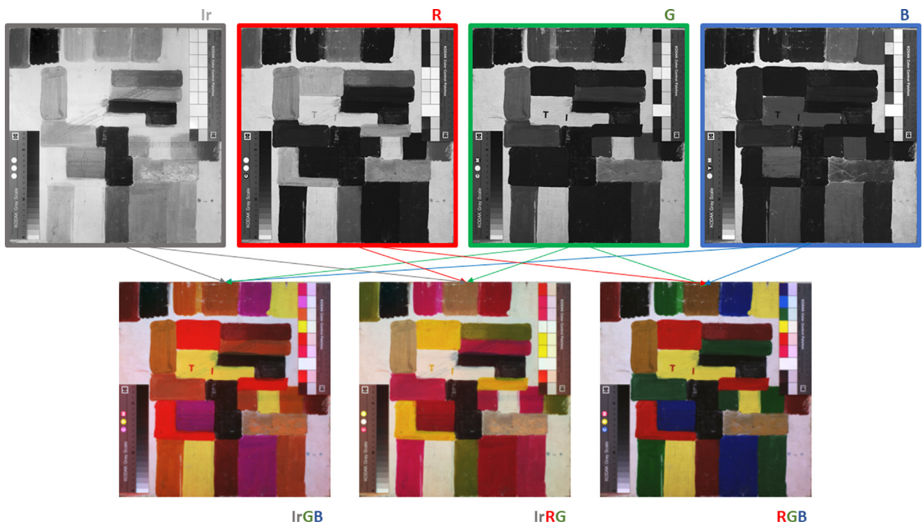
Fig. 5. Schematic representation of the procedure used for building lrRG and lrGB false colour images from a multispectral set of images.
