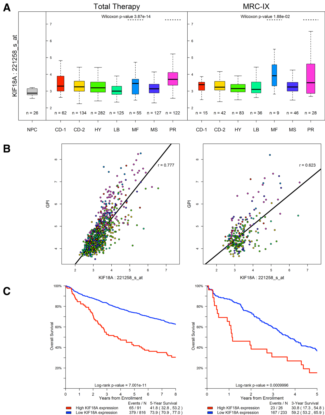
Figure 1: KIF18A expression in the Total Therapy and MRC-IX (MRC Myeloma-IX) trials. (A) KIF18A expression for the seven established MM molecular subtypes [27]. TC classification groups are generated by molecular classification of patients based on unsupervised hierarchical clustering. Y-axis denotes normalized \log_2 KIF18A expression. On the boxplot the width of the boxes corresponds to the group size; the thick black line to the median; the vertical extremities of the boxes correspond to the lower and upper quartiles. The CD-1 and CD-2 groups relate to IgH translocation cases with activating CCND1 or CCND3 , the CD-2 group is distinguished from CD-1 by the expression of CD20 and PAX5 . MS group defines upregulation of FGFR3 and/or MMSET , whilst the MF group is characterized by c-MAF or MAFB . LB group is defined by a low number of bone lesions. HY group that contains HD cases and PR group is characterized by the overexpression of cancer-testis antigens, cell cycle and proliferation-related genes. KIF18A is significantly highly expressed in subtypes MF and PR. The level of expression of KIF18A in normal plasma cells (NPC) is shown. (B) Relationship between gene expression-based proliferation index [7] (GPI) and KIF18A expression. (C) KIF18A expression and prognosis in MM. High expression (top 10%) of KIF18A is significantly associated with worse survival in the Total Therapy trial, and the MRC-IX trial data exhibits the same trend.
