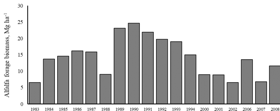
Fig. 2. Means of annual alfalfa forage biomass production in the field trials throughout the data collection period from 1983 to 2008.
