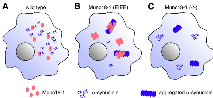
Figure 1. Munc18-1 acts as a chaperone for \alpha -synuclein. (A) Healthy cells. (B) E1EE-linked mutants in Munc18-1 cause haploinsufficiency by seeding aggregation of wild-type Munc18-1 and causing aggregation of \alpha -synuclein. (C) \alpha -Synuclein aggregates in the absence of Munc18-1.
