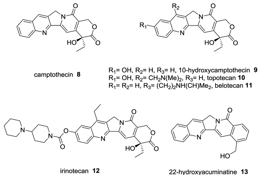
Fig. 3 Structures of natural alkaloids and anticancer drugs.
