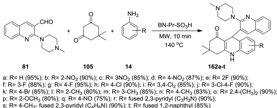
Scheme 56 Synthesis of piperazinyl-quinolinyl-acridinone systems.
