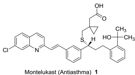
Fig. 1 Structure of antiasthma agent incorporating quinoline nucleus.
