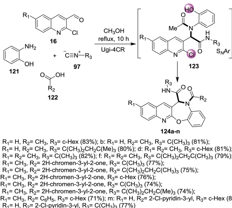
Scheme 40 Synthesis of benzo[2,3][1,4]oxazepino[7,6- b ]quinolines.
