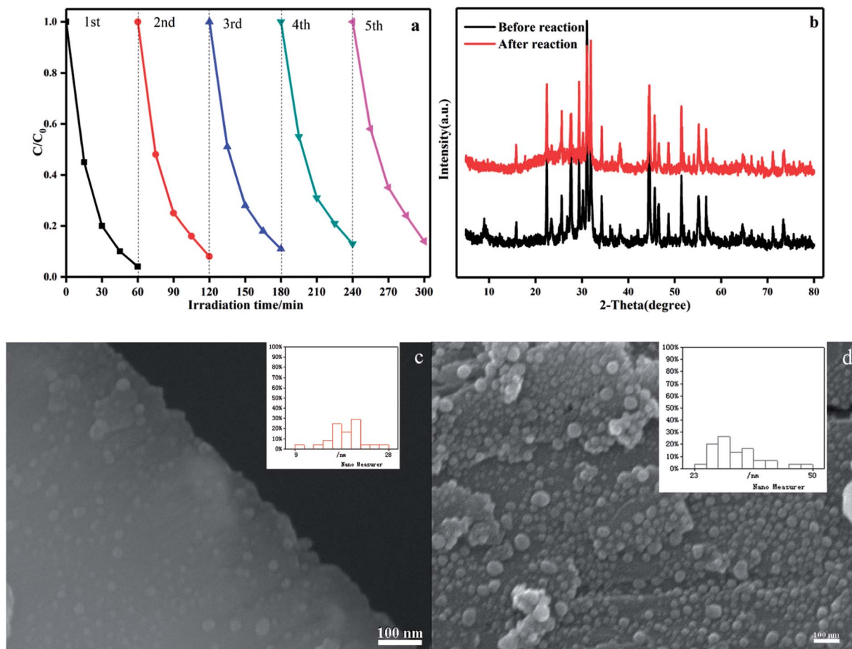
Fig. 11 (a) Cycling runs for photocatalytic degradation of MB in the presence of Ag@AgBr/ K_4Nb_6O_{17} . (b) XRD patterns of Ag@AgBr/ K_4Nb_6O_{17} before and after the photocatalytic reaction. (c and d) SEM images of photocatalysts before and after photocatalytic degradation of MB solution.
