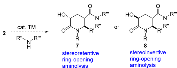
D: Prior report on site-selective deconstructive amination of a \beta -lactone
