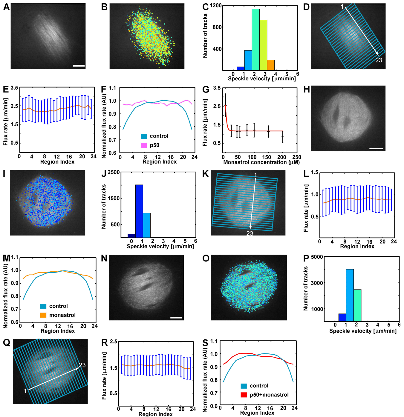
Figure 3. Inhibition of dynein/dynactin, kinesin-5, or both suppresses regional variation of poleward microtubule flux. (A) Spindle treated with excess p50/dynamitin. (B and C) Speckle trajectories color coded according to the velocity histogram (C); the flux rate of the specific spindle shown is mean \pm SD = 2.33 \pm 0.60 \mu\text{m}/\text{min} ( n = 2,702 trajectories). (D and E) Mean and SD (error bars) of speckle velocities within regions in D. (F) Normalized flux rate along the pole-to-pole axis of control (average over 11 spindles) versus p50/dynamitin-treated spindles (average over seven spindles). (G) Flux rates at different monastrol concentrations. (H) Spindle treated with 200 \mu\text{M} monastrol. (I and J) Speckle trajectories color coded according to the velocity histogram (J); the flux rate of the spindle shown is mean \pm SD = 0.89 \pm 0.30 \mu\text{m}/\text{min} ( n = 3,085 trajectories). (K and L) Mean and SD (error bars) of speckle velocities within regions in K. (M) Normalized flux rate distribution along the pole-to-pole axis of control and monastrol-treated spindles (average over 17 spindles treated with 20–200 \mu\text{M} monastrol). (N) Spindle treated with both 200 \mu\text{M} monastrol and excess p50/dynamitin. (O and P) Speckle trajectories color coded according to the velocity histogram (P); the flux rate of the spindle shown is mean \pm SD = 1.59 \pm 0.38 \mu\text{m}/\text{min} ( n = 7,214 trajectories). (Q and R) Mean and SD (error bars) of speckle velocities within regions in Q. (S) Normalized flux rate distribution along the pole-to-pole axis of control versus monastrol + p50/dynamitin-treated spindles (average over six spindles). Bars, 10 \mu\text{m} .
