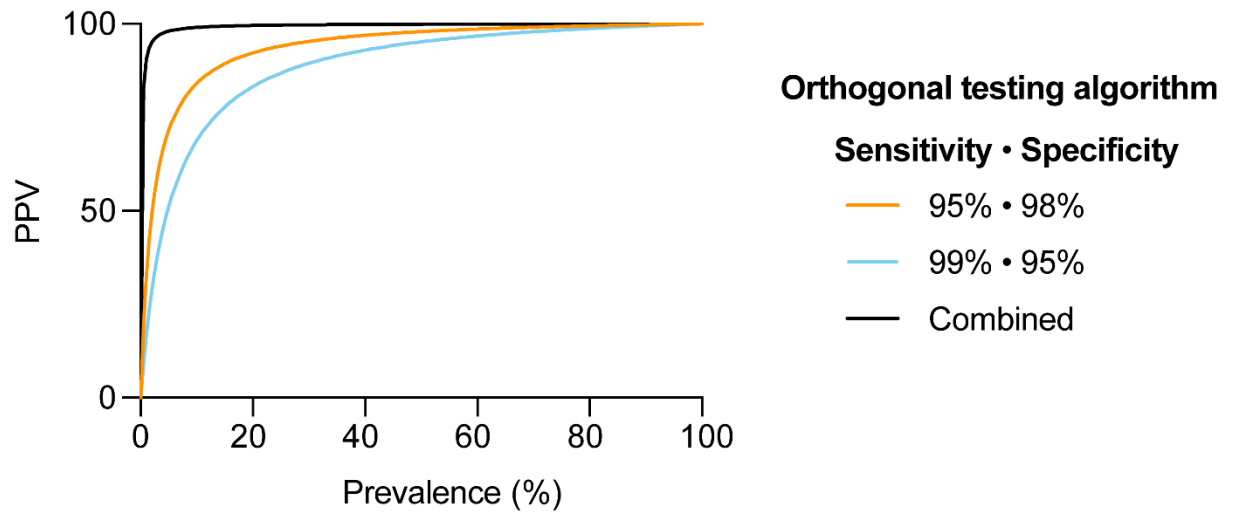
Figure 4. Effect of an Orthogonal Testing Algorithm (OTA) on Positive Predictive Value (PPV). Shown is the performance of two tests with different characteristics (Test 1: sensitivity, 95%; specificity, 98%. Test 2: sensitivity, 99%; specificity, 95%) and their combined performance. Regardless of the order in which the tests are performed, sequential testing can increase PPV in testing populations with low disease prevalence.
