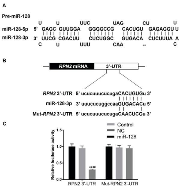
Figure 6. Binding site prediction and luciferase report assay. (A) The cervical-loop structures of miR-128. (B) Putative targets predicted by Target Scan. (C) Relative luciferase activity resulted from binding of RPN2 3'-UTR reporter and miR-128. *** P<0.01 vs. control, ** P<0.01 vs. NC. miR, microRNA; RPN2, Ribophorin-II; UTR, untranslated region; NC, negative control; Mut, mutant.
