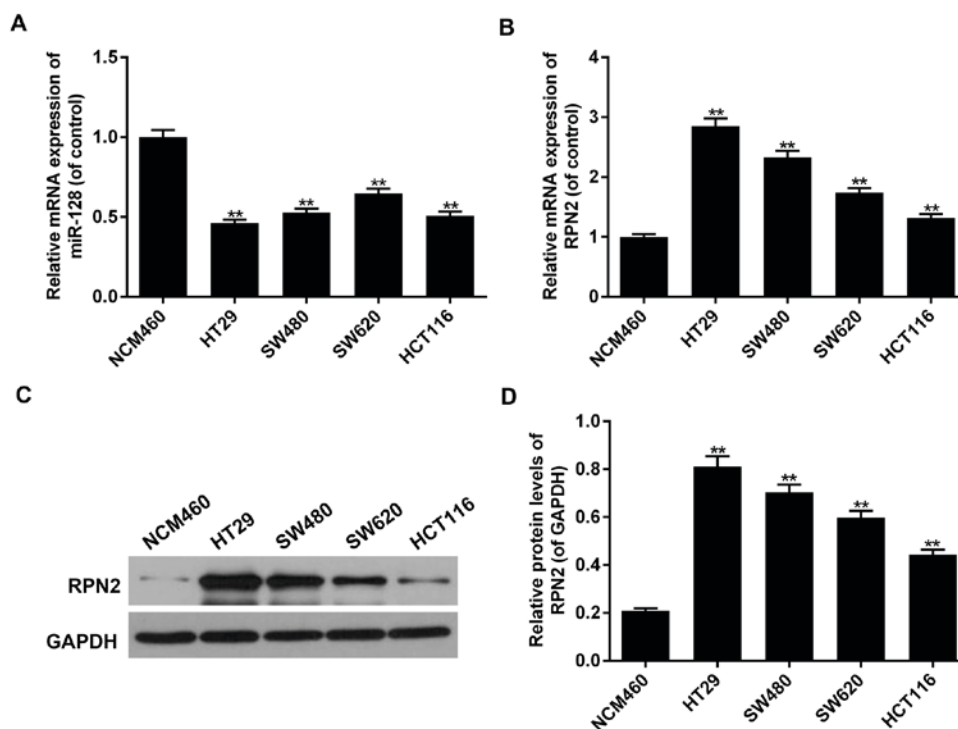
Figure 2. Expression of miR-128 and RPN2 in CRC HT29, SW480, SW620 and HCT116 cell lines was assessed. (A) The miR-128 levels in CRC cell lines were significantly decreased, compared with the normal NCM460 cell line. (B) The mRNA levels of RPN2 in CRC cell lines were significantly increased, compared with normal NCM460 cells. (C) Western blot analysis of RPN2 protein expression in CRC and normal cell lines. (D) The protein levels of RPN2 in CRC cell lines were significantly increased compared with normal NCM460 cells. Data are expressed as the mean \pm standard deviation from three independent experiments. ** P < 0.01 vs. normal cells. RPN2, Ribophorin-II; CRC, colorectal cancer.
