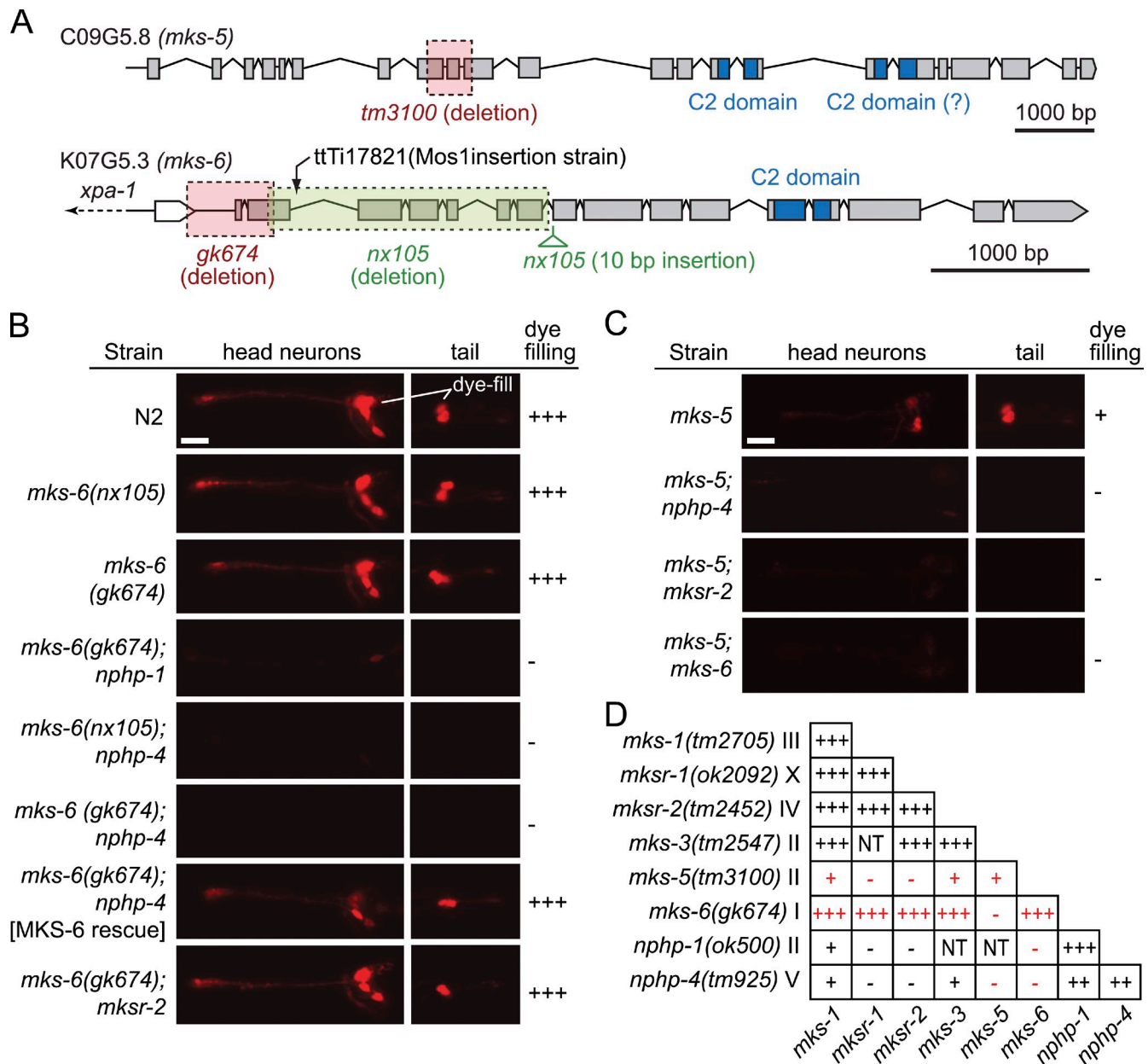
Figure 3. Functional interactions between MKS-5/MKS-6 and other TZ proteins are required for environmental exposure of cilia to a fluorescent dye, consistent with a role in ciliogenesis. (A) Gene structures of C. elegans mks-5 (C09G5.8) and mks-6 (K07G5.3) and the nature of three deletion alleles, tm3100 , gk674 , and nx105 . (B and C) Representative images of fluorescence staining of environmentally exposed sensory neurons via Dil uptake through cilia in head (amphid) neurons (left panels) and tail (phasmid) neurons (right panels). Dye filling is noted as normal (+++), reduced (+), or absent (-). (B) Wild-type (N2) and mks-6 strains exhibit normal dye filling; nphp-1 and nphp-4 show normal or slightly reduced (++) dye filling (see D; Jauregui et al., 2008). mks-6;mks-5 , mks-6;nphp-1 , and mks-6;nphp-4 double-mutant combinations show little or no dye filling. Expressing GFP-tagged MKS-6 rescues the mks-6 (double) mutant phenotype. (C) mks-5(tm3100) mutants have reduced dye filling, whereas mks-5;mksr-2 , mks-5;mks-6 , and mks-5;nphp-4 double mutants show little to no dye filling. Bars, 17.5 \mu m. (D) Summary of dye-filling phenotypes in single and double mks/mksr/nphp mutants. NT, not tested; red, present study; black, data from Jauregui et al. (2008) and Williams et al. (2008, 2010).
