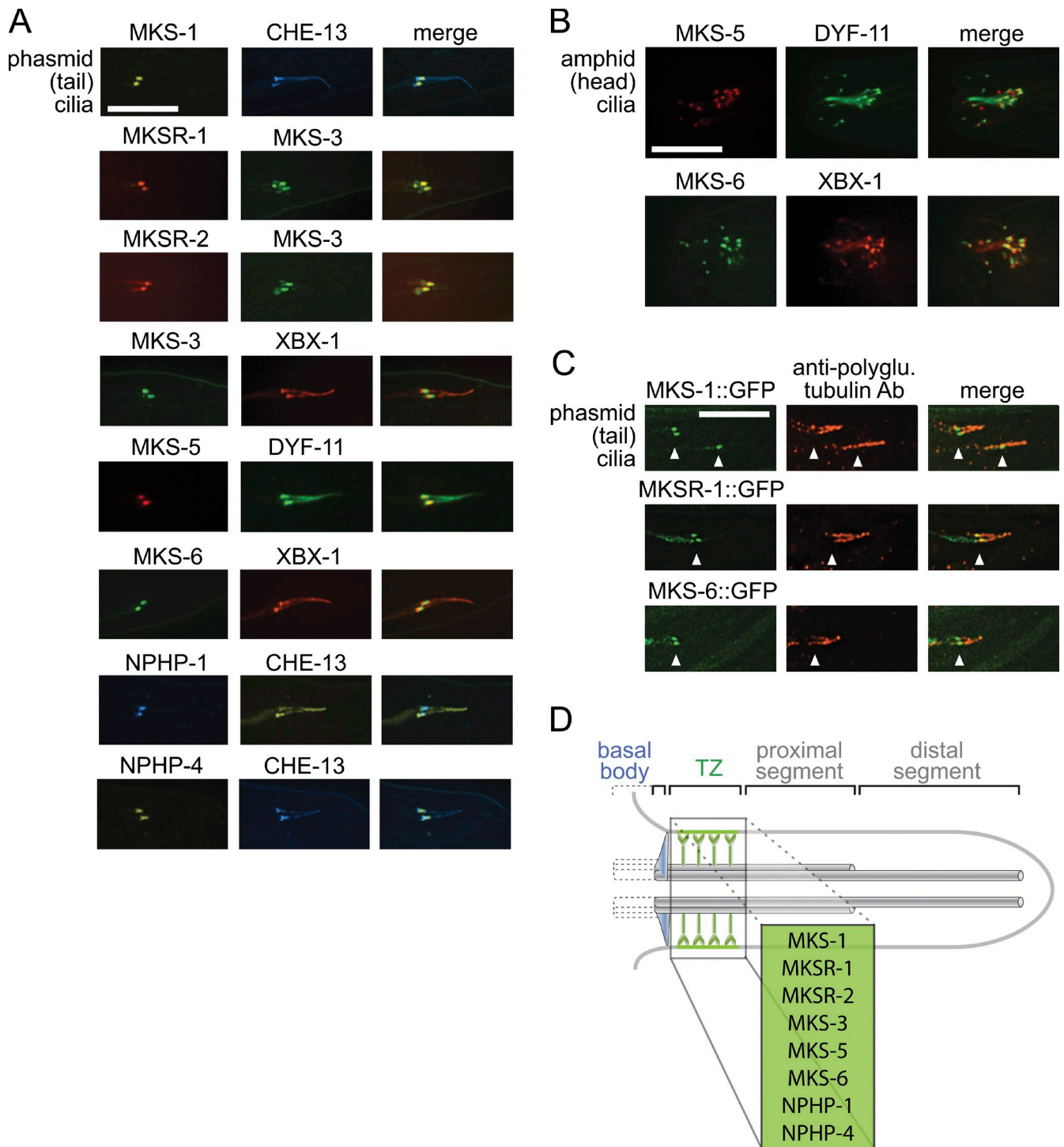
Figure 2. MKS/MKSR and NPHP proteins localize at the ciliary TZ. (A) Fluorophore-tagged MKS/MKSR and NPHP proteins localize at the TZ in tail cilia. Each TZ protein signal is overlaid with IFT or other TZ protein signal, as indicated. Bar, 10 \mu m. (B) MKS-5::tdTomato and MKS-6::GFP localize at the TZ in head cilia. MKS-5 and MKS-6 are overlaid with IFT proteins DYF-11::GFP and XBX-1::tdTomato, respectively. Bar, 10 \mu m. (C) GFP-tagged MKS-1, MKSR-1, and MKS-6 localize at the base of ciliary axonemes (consistent with the TZ), which are marked by staining with an antibody against polyglutamylated tubulin. Bar, 10 \mu m. (D) Schematic of MKS/MKSR/NPHP protein localization at the TZ.
