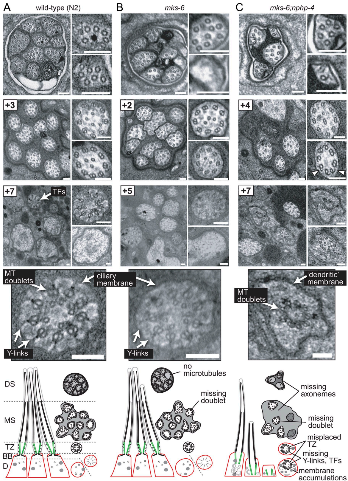
Figure 6. MKS-6 and NPHP-4 are collectively required for BB/TZ attachments to membrane. Shown are low and high magnification images from TEM serial cross sections of amphid channel cilia from wild-type (N2), mks-6 , and mks-6;nphp-4 worms. Top row, distal segments (DS); middle row, middle segments (MS); bottom row, transition zone (TZ) and distal dendrites (DD). Below bottom row are magnified images of representative TZs. Boxed number denotes proximal positioning of section relative to top section. BB, basal body; TFs, transition fibers. Bars, 100 nm. (A) N2 worms showing 10 singlet microtubule (MT)-containing axonemes in DS, 10 doublets in MS (+3 \mu m), and TZs (constriction of MT doublets surrounding apical ring) with intact Y-links (connecting doublets with ciliary membrane) anchored at distal dendrite tips (+7 \mu m). TFs are also observed below this region. (B) Apart from rare axonemes lacking MTs in DS, mks-6 mutant cilia possess normal DS,
