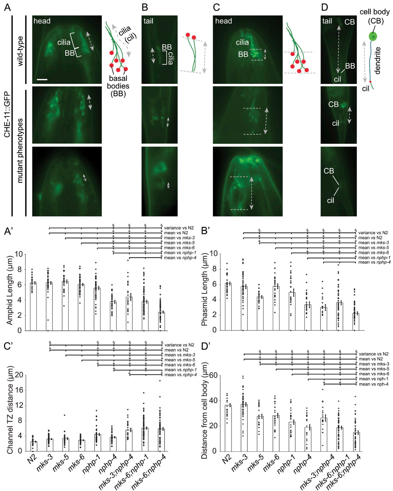
Figure 5. Detailed analysis of cilia length and positioning in strains with disrupted TZ proteins. (A–D) Example of correct (wild type; top panels) or defective (for TZ gene mutants; bottom two panels) amphid (A) and phasmid (B) cilia length, distribution of BBs in amphid ciliated neurons (C), and positioning of the BB with respect phasmid neuron cell body (D), using a CHE-11::GFP IFT marker (with the exception of the mks-5 data, which was obtained using OSM-6::GFP). CB, cell body; cil, cilia; BB, basal body. Bar, 5 \mu\text{m} . (A'–D') Individual data points ( n > 40 ) of the measurements in A–D are shown with a bar graph showing average and standard error. Statistically significant differences ( P < 0.01 ) in the mean (*) or variance (§) are indicated for all combinations.
