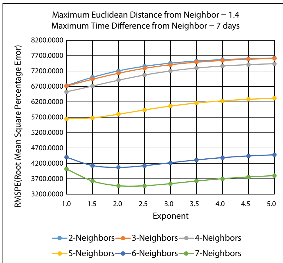
Figure 21. RMSPE 10-fold cross-validation results for the various 45 IDW methods using the improved IDW interpolation.
