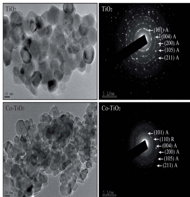
Fig. 2 (left panel) TEM images of un-doped TiO 2 and 5 at% Co-doped TiO 2 NPs. (right panel) SAED images of un-doped TiO 2 and 5 at% Co-doped TiO 2 NPs.
