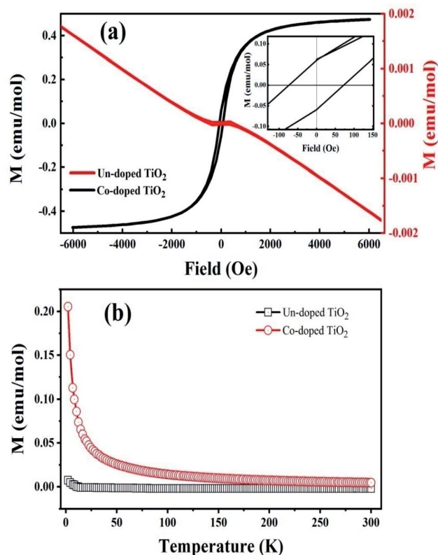
Fig. 5 (a) Room temperature M - H loops of the un-doped and 5 at% Co-doped TiO 2 NPs. (b) Magnetization vs. temperature curves of the studied samples.
