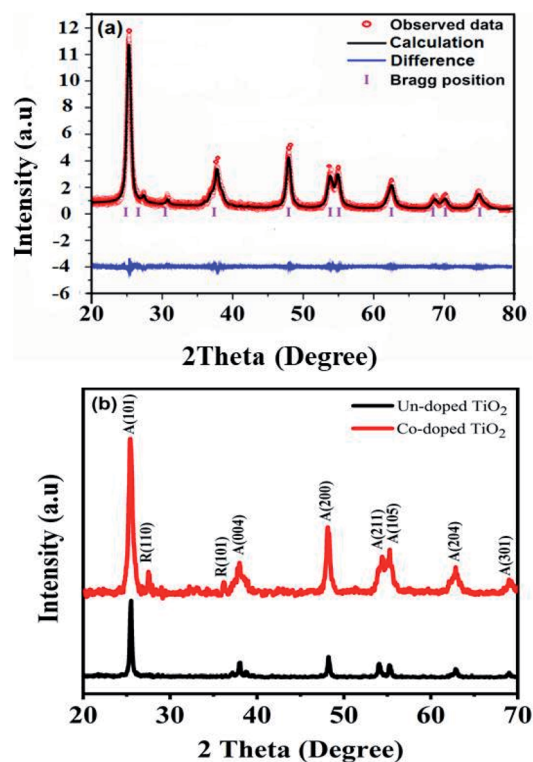
Fig. 1 (a) X-ray diffraction pattern of TiO 2 NPs with its Rietveld refinement. (b) XRD patterns of un-doped and 5 at% Co-doped TiO 2 NPs; the inset in the figure shows the peak shifting with Co-doping.
