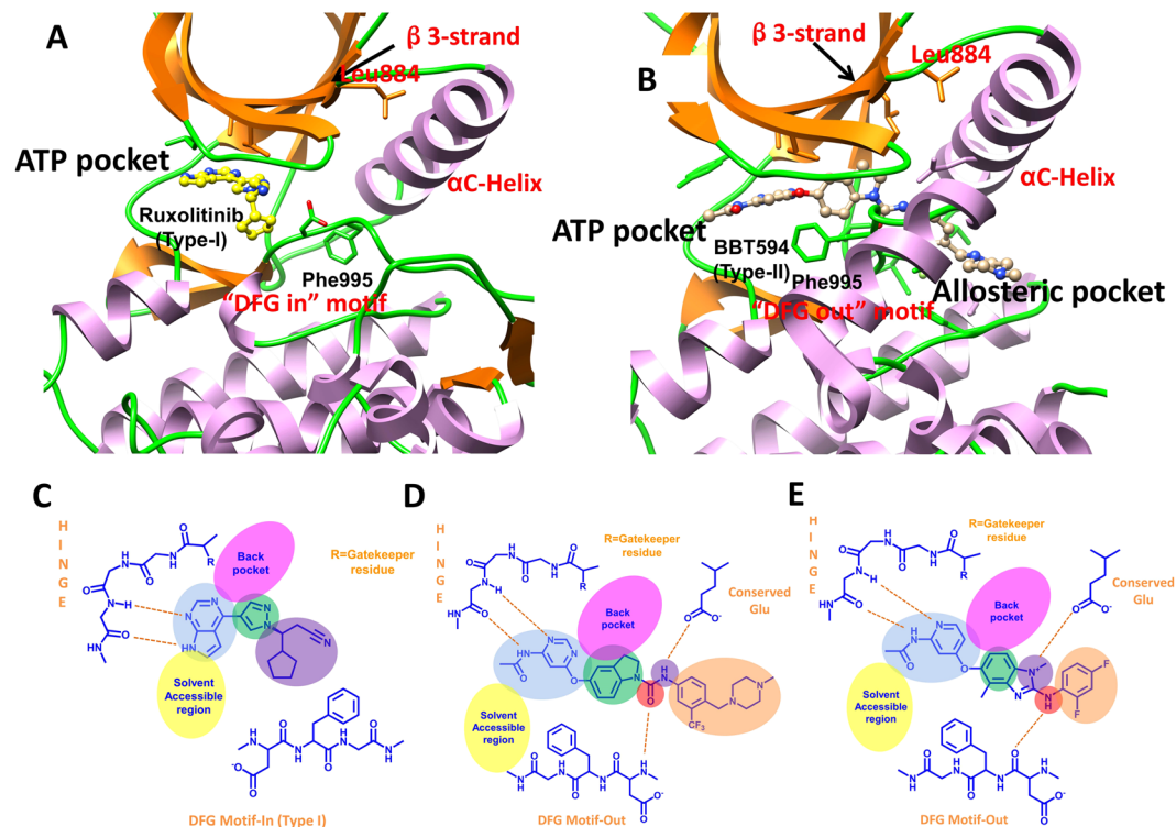
Figure 1. Type-I inhibitor Ruxolitinib bound to JAK2 with the DFG-in conformation (PDB code: 4U5), panel A), and Type-II inhibitor BBT594 bound to JAK2 with the DFG-out conformation (PDB entry: 3UGC, panel B). The 2D-interactions between JAK2 and Ruxolitinib, BBT594, and CHZ868 are shown in panels C~E.
