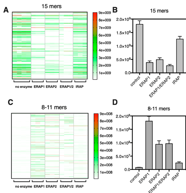
Figure 1. (A) Heatmap showing trimming of 15mers by amino-peptidases for each biological replicate. (B) Average label-free quantification (LFQ) signal of 15mers in the sample before and after incubation with the indicated enzyme. (C) Heatmap showing LFQ signal for 8–11mers produced after digestion. (D) Average LFQ signal of 8–11mers.
