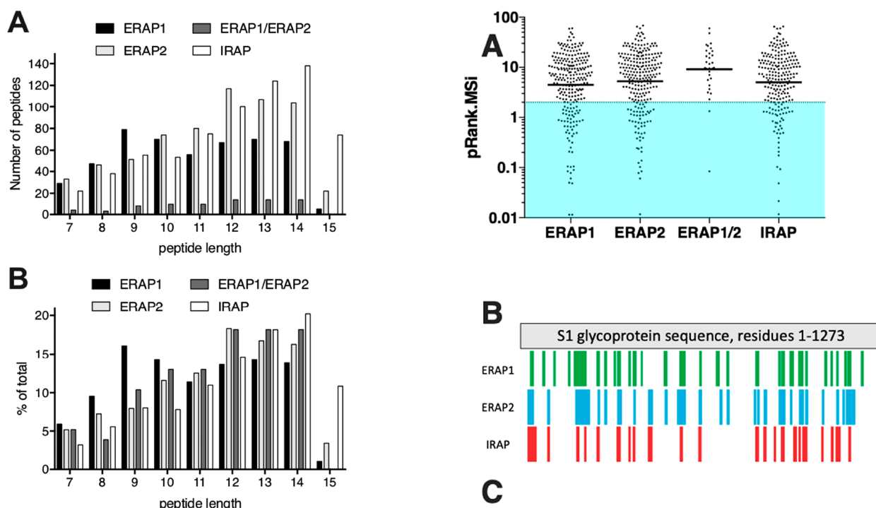
Figure 3. Length distribution of peptides detected by LC-MS/MS after enzymatic digestion. (A) Number of peptides detected of each length. (B) Relative fraction of each length compared to the total number of peptides detected.
