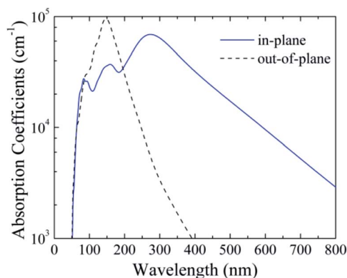
Fig. 4 Calculated in-plane and out-of-plane absorption coefficients of silicether with the HSE06 method.
