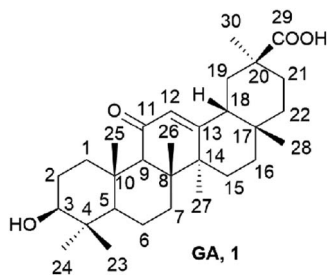
Fig. 1 Structures of 18 \beta -glycyrrhetic acid (GA).
