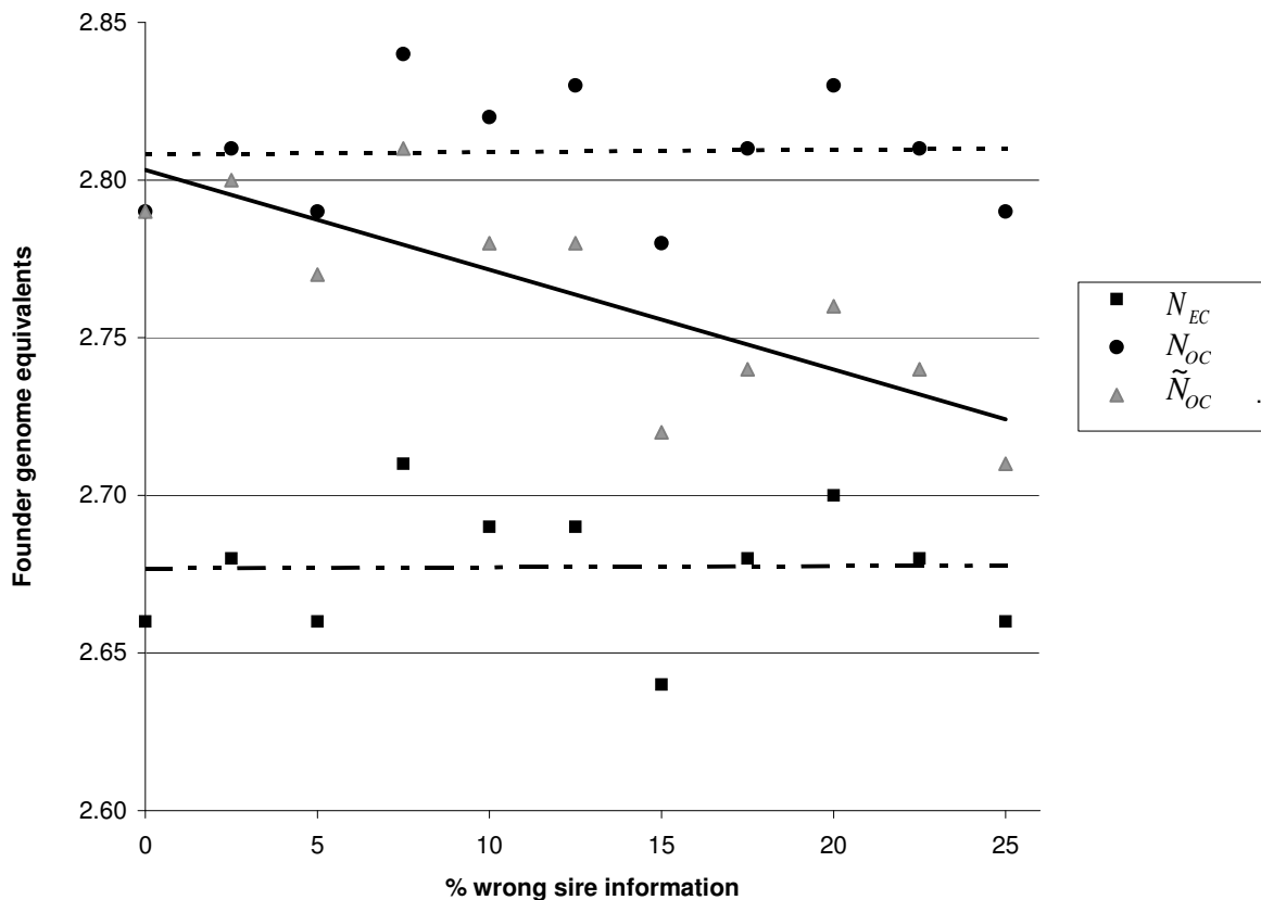
Figure 1 Diversity in a panmictic population with wrong sire information. Results are averages of 200 replicates of the standard population. Standard errors of results were 0.02. Trend lines are added for each legend entry. N_{EC} is Founder genome equivalent of the average kinship (achieved by applying equal contributions). N_{OC} is Founder genome equivalent of the average kinship achieved by applying optimal contributions based on true pedigrees. \tilde{N}_{OC} is Diversity Criterion, the founder genome equivalent of the average kinship achieved by applying optimal contributions based on observed pedigrees.
