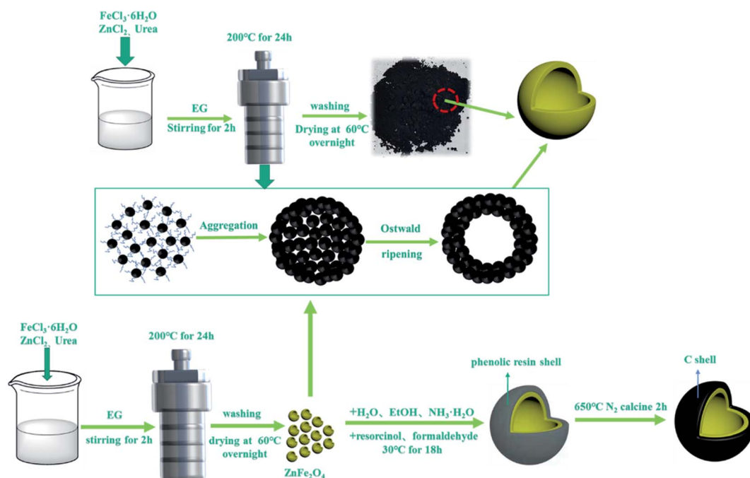
Fig. 1 Schematic illustration of the process for the synthesis of hollow core-shell \text{ZnFe}_2\text{O}_4@C composites.
