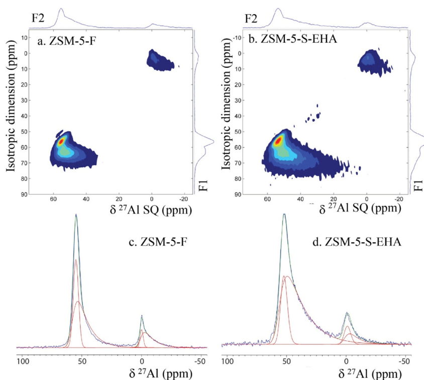
Figure 1. Top: ^{27}\text{Al} 3QMAS NMR spectra of: a) zeolite ZSM-5-F and b) zeolite ZSM-5-S-EHA. The 2D spectra are sheared so that the projection on the F1 axis gives an isotropic spectrum. Bottom: Normalized ^{27}\text{Al} MAS NMR spectra of: c) zeolite ZSM-5-F and d) zeolite ZSM-5-S-EHA (blue: experimental, green: fitted, red: simulated peaks).
