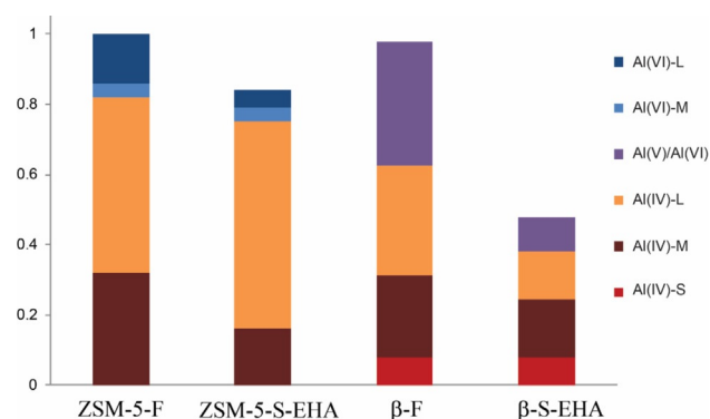
Figure 3. Relative amounts of four-, five-, and six-coordinated aluminum species in zeolites ZSM-5-F, ZSM-5-S-EHA, \beta -F and \beta -S-EHA, normalized to the total aluminum content in zeolite ZSM-5-F, as determined by ^{27}\text{Al} MAS NMR (accuracy \pm 2\% ).
