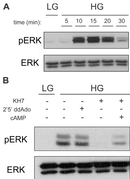
Figure 6. Glucose leads to ERK (p42/44) activation in a sAC-dependent manner. Western blots using anti-phosphoERK (pERK) or total ERK (ERK) of INS-1 cells incubated in Krebs Ringer buffer with 2.5 mM glucose (LG) or 16 mM glucose (HG) (in the absence of IBMX) (A) for 5, 10, 15, 20, and 30 min or (B) for 15 min in the presence or absence of 30 \mu M KH7 or 50 \mu M 2'5' ddAdo or KH7 and 0.5 mM Sp-8Br-cAMP. Western blot shows phosphorylation and total protein for both ERK1 and ERK2, p44 and p42. Shown are representative experiments repeated multiple times (for A, n = 4 ; for B, n = 7 ).
