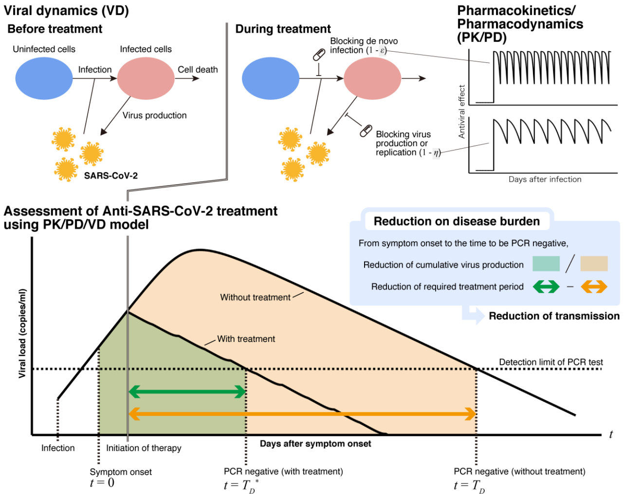
Fig. S3. Schematic representation of SARS-CoV-2 infection dynamics, related to Figure 7. A typical disease progress with viral load on patients undergoing therapy are shown. The outcomes for the therapies, that is, reduction in “period until virus elimination” and “cumulative virus production” are graphically depicted.
