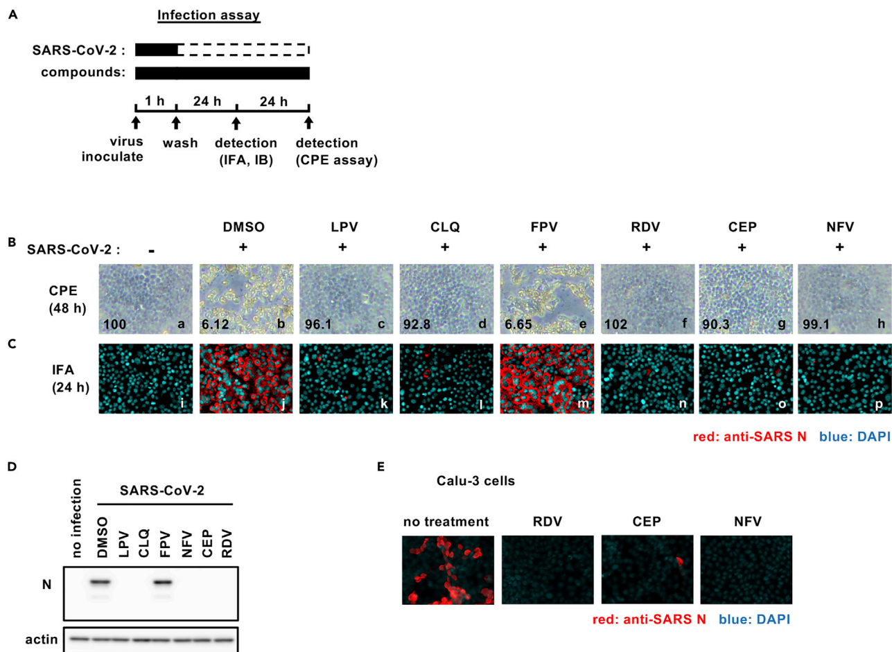
Figure 1. Cepharranthine (CEP) and nelfinavir (NFV) inhibit SARS-CoV-2 infection
