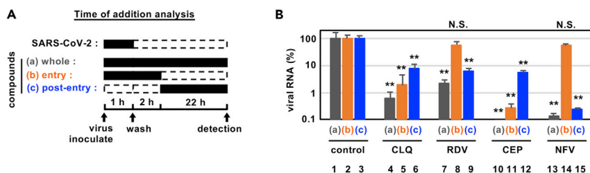
Figure 3. Antiviral mechanism of action for CEP and NFV
