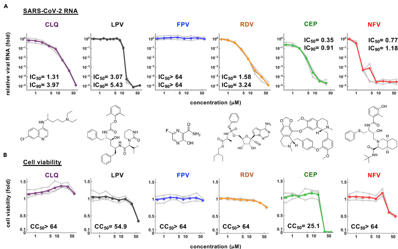
Figure 2. Dose-response curves for the antiviral activity of CEP and NFV
