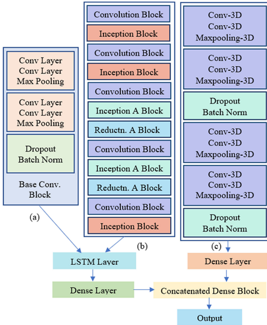
FIGURE 2 Ensemble model: (a) 2D convolutional neural network (CNN) LSTM, (b) 2D CNN LSTM with Inception V4 Modules, and (c) 3D CNN.
