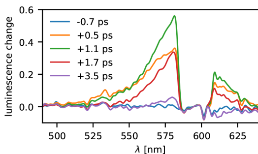
Figure 6. Difference spectra from Figure 4f. In order of increasing \tau , the state before the pump pulse, the highest \tilde{T}_{\text{e}} state ( \tau = +0.5 ps), the highest intensity state ( \tau = +1.1 ps), a slightly later state ( \tau = +1.7 ps), and a late- \tau state.
