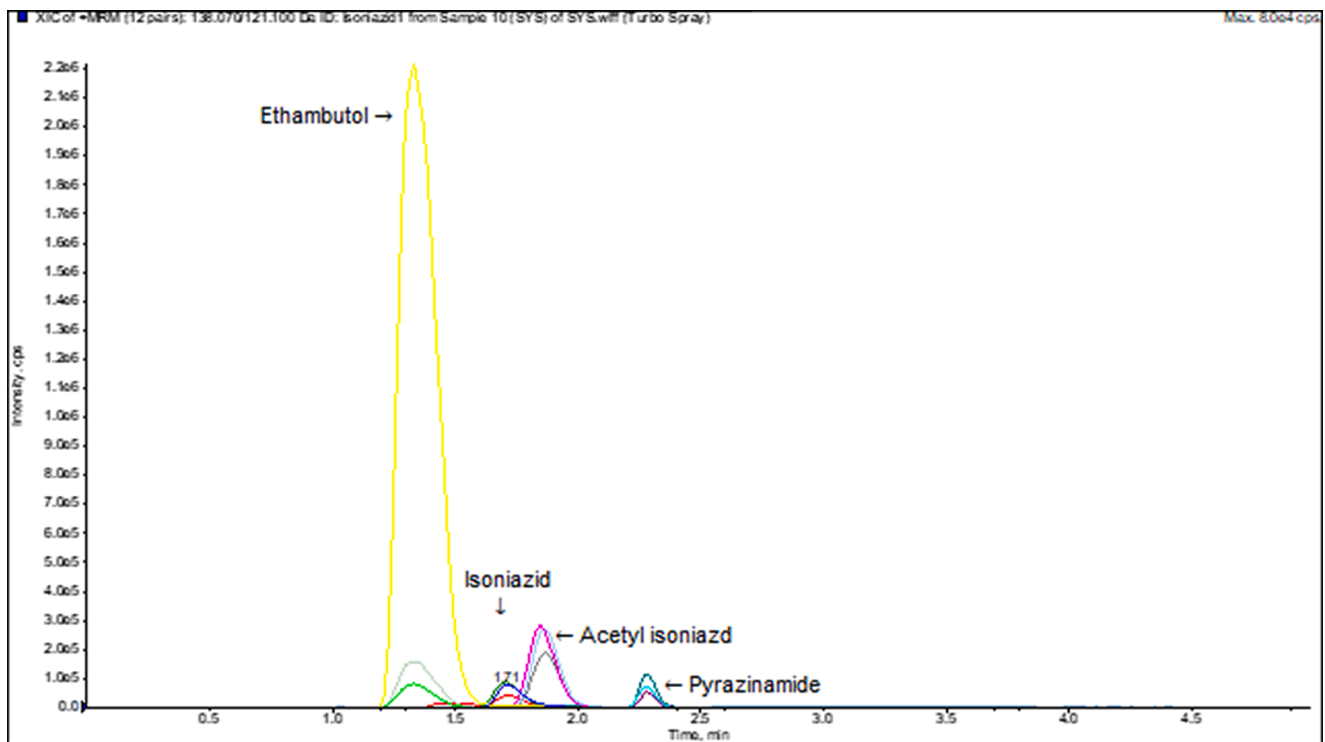
Fig. 1. Chromatographic representation of the small more polar analytes showing two transitions for each analyte and their respective internal standards at concentrations of 6.01 \mu\text{g/mL} , 3.00 \mu\text{g/mL} , 6.01 \mu\text{g/mL} , and 3.00 \mu\text{g/mL} for isoniazid, acetyl isoniazid, ethambutol, and pyrazinamide, respectively.
