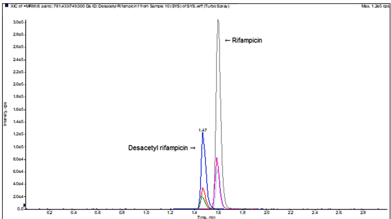
Fig. 2. Chromatographic representation of rifampicin and desacetyl rifampicin showing two transitions for each analyte and their respective internal standards at a concentration of 3.00 \mu\text{g/mL} for both rifampicin and desacetyl rifampicin.
