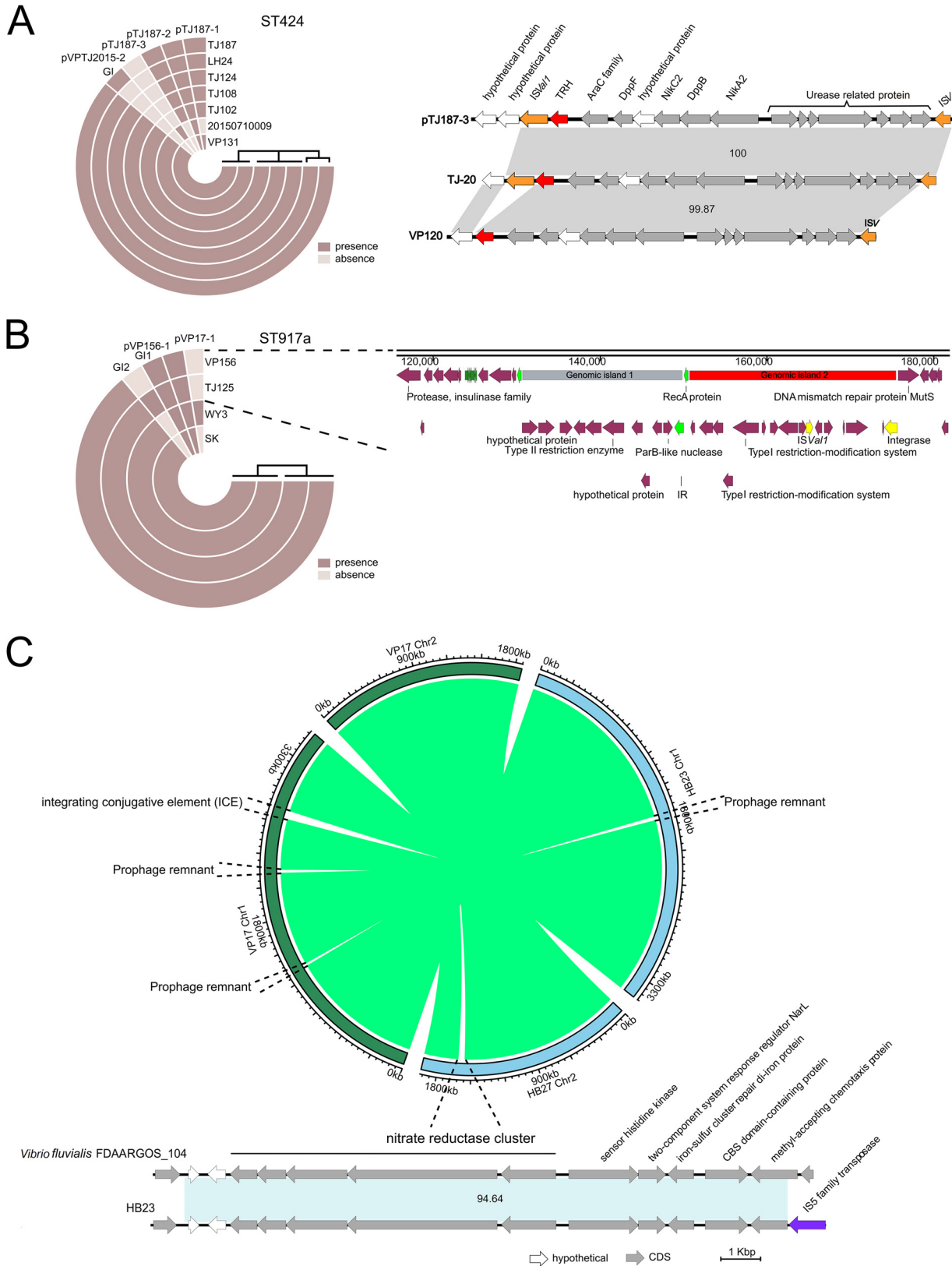
FIG 4 Horizontal transfer of a genomic island. (A) Horizontal transfer of a thr-nik-ure genomic island from the chromosome to the plasmid mediated by ISVal1 . (B) Schematic diagram showing the comparative genome analysis of ST917a isolates and the integration of two genomic islands near reC in VP156 and TJ125. (C) Comparative genome analysis between the V. parahaemolyticus strain VP17 and HB23. Linear comparison of an inserted genomic island between V. parahaemolyticus genome HB23 and Vibrio fluvialis genome FDAARGOS_104 showing the acquisition of a nitrate reductase cluster.
