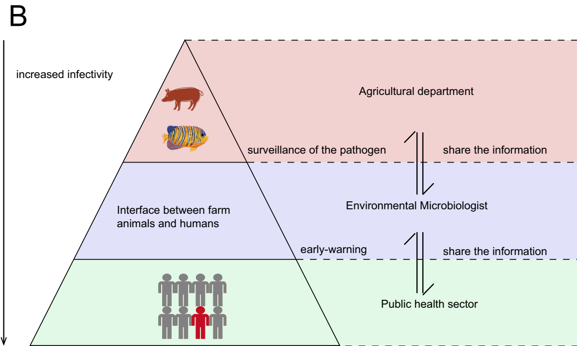
FIG 6 (A and B) Four milestone evolutionary stages of bacterial pathogens (A) and suggested prevention strategies (B). Evolutionary trajectories were divided into the following four stages: stage 1, transfer of ISVal1 from plasmid to chromosome; stage 2, formation of resistant MGEs; stage 3, formation of virulent MGEs; stage 4, horizontal transfer of MGEs and plasmid. The decline of the outbreak-related pond is due to the discarding of the pond.
