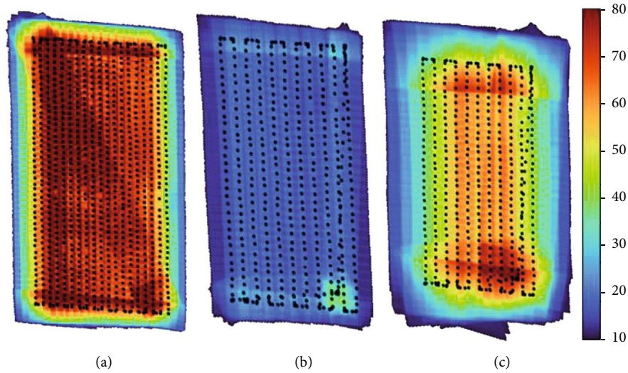
FIGURE 3: Camera positions (black dots) and number of images per pixel of orthoimage for (a) SS f = 8 mm (green band), (b) DS f = 8 mm (green band), and (c) DS f = 4.2 mm (far green band). The color bar on the right represents the number of images of each pixel of orthoimage that was averaged over 0.5 \text{ m} \times 0.5 \text{ m} cells.
