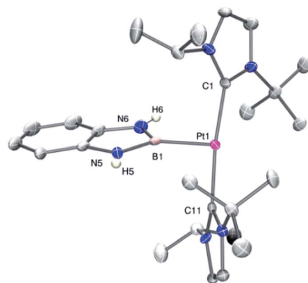
Fig. 1 ORTEP representation of the cation of complex 2c . Hydrogen atoms (except those of the NH moieties) have been omitted for clarity. Selected bond distances (Å) and angles (°): Pt1–B1, 1.988(6); Pt1–C1, 2.015(5); Pt1–C11, 2.016(5); B1–N6, 1.424(7); B1–N5, 1.433(7); C1–Pt1–C11, 173.5(2); B1–Pt1–C1, 92.9(2); B1–Pt1–C11, 93.6(2).
