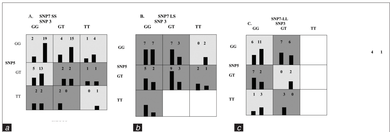
Figure 1: (a–c) The best three-locus SNP model selected by MDR. interaction of NOS3 G894T, 5HTT , and EDN1 K198N polymorphisms
