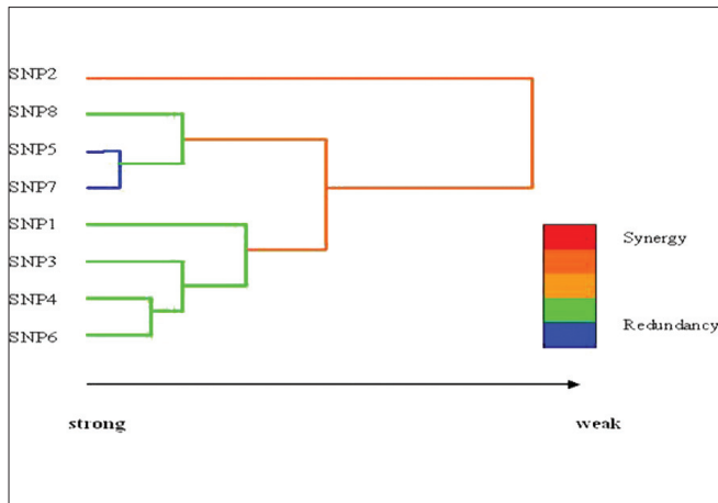
Figure 2: The dendrogram demonstrates the nature of the interactions between SNPs. The colors used in the dendrogram comprise of a spectrum of colors representing a continuum from synergy to redundancy. Red denotes a high degree of interaction, orange denotes a lesser degree of interaction, and green denotes a weak interaction. Blue lines indicate no interaction or redundancy
