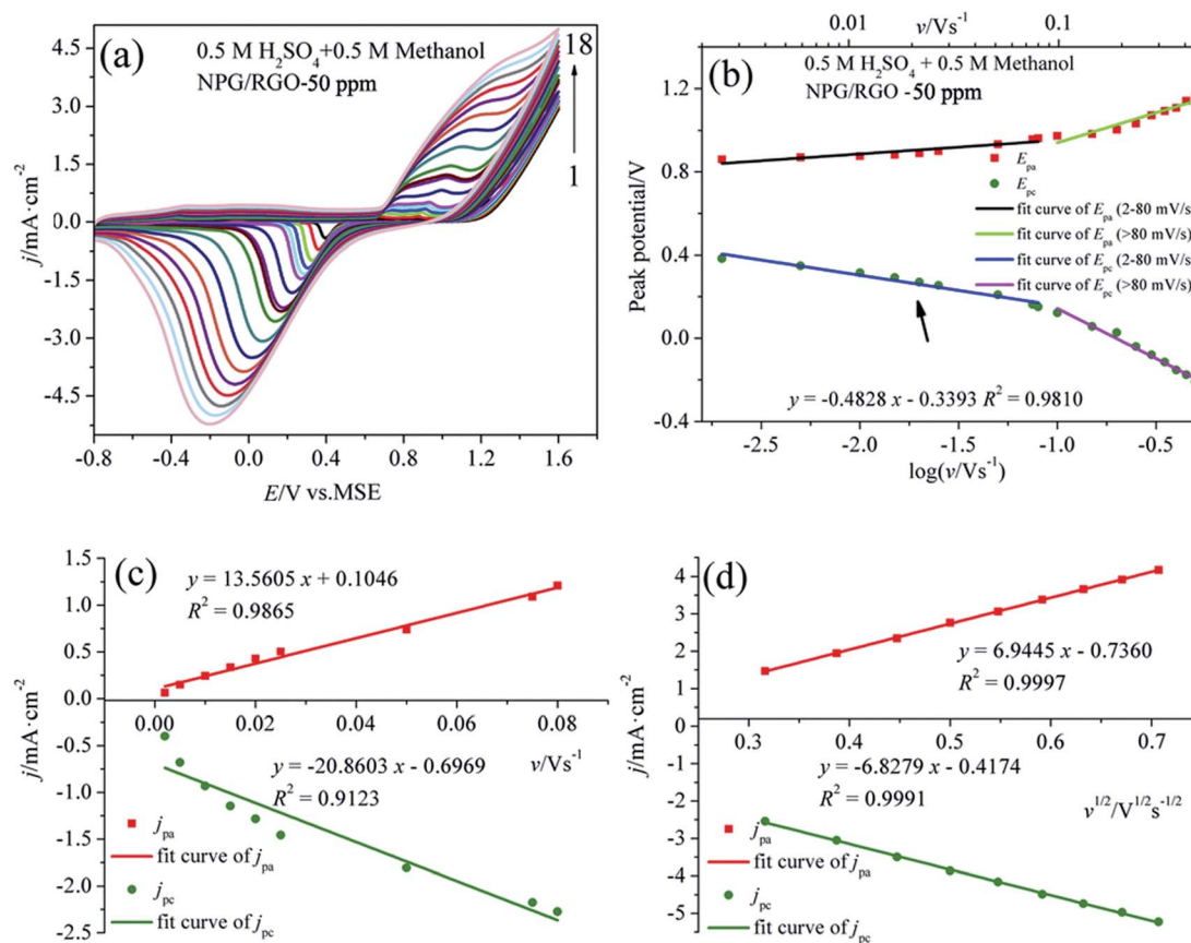
Fig. 8 (a) CVs of S1 electrode in 0.5 M H 2 SO 4 + 0.5 M methanol solution at various scan rates v , (b) plot of E_p vs. \log v for anodic and cathodic peaks, (c) dependency of j_{pa} and j_{pc} on lower values of v and (d) on v^{1/2} at higher values of v .
