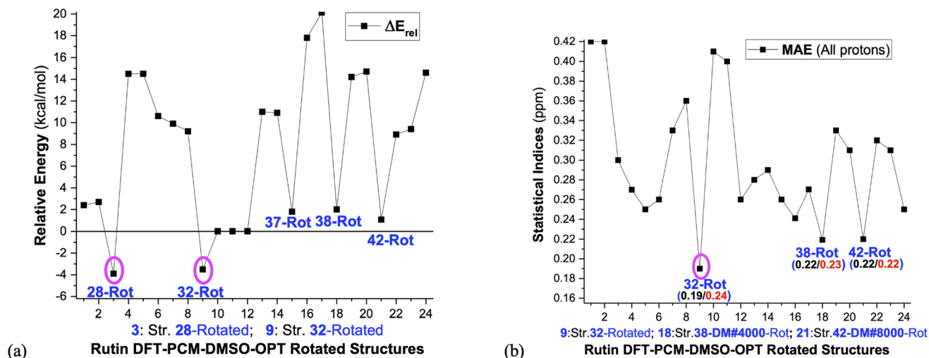
Fig. 2 (a) \omega B97X-D/6-31G(d,p)-PCM-DMSO relative energies ( \Delta E_{rel} and \Delta G_{rel} in kcal mol -1 ) with respect to structure 34 (b) B3LYP/6-31G(d,p)-PCM-DMSO statistical indices (MAE in ppm) values with all protons included and using only the sugar moiety protons are given. \Delta G_{rel} was estimated using thermal corrections for DFT fully optimized structures (the \phi_1 , \phi_2 rotated structures are not true minimum on the PES, so harmonic frequency calculations, needed for evaluation of thermal correction, are meaningless). The torsion angles for \phi_1 , \phi_2 rotated structures are given in Table 1. 1: Str-28-PCM-OPT; 2: Str-28 Vacuum-OPT; 3: Str-28-PCM-OPT-Rotated; 4: Str-30-PCM-OPT; 5: Str-30 Vacuum-OPT; 6: Str-30-PCM-OPT-Rotated; 7: Str-32-PCM-OPT; 8: Str-32 Vacuum-OPT; 9: Str-32-PCM-OPT-Rotated; 10: Str-34-PCM-OPT; 11: Str-34 Vacuum-OPT; 12: Str-34-PCM-OPT-Rotated; 13: Str-37-PCM-OPT; 14: Str-37 Vacuum-OPT; 15: Str-37-PCM-OPT-Rotated; 16: Str-38-PCM-OPT; 17: Str-38 Vacuum-OPT; 18: Str-38-PCM-OPT-Rotated; 19: Str-42-PCM-OPT; 20: Str-42 Vacuum-OPT; 21: Str-42-PCM-OPT-Rotated; 22: Str-44-PCM-OPT; 23: Str-44 Vacuum-OPT; 24: Str-44-PCM-OPT-Rotated.
