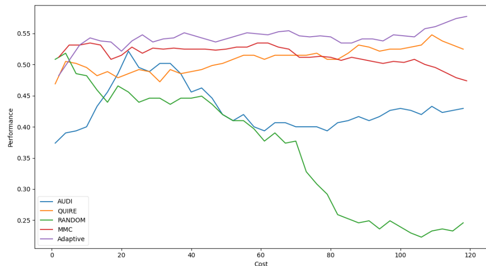
Figure 5. Classification accuracy for the five selection AL strategies without grid search optimizer.
