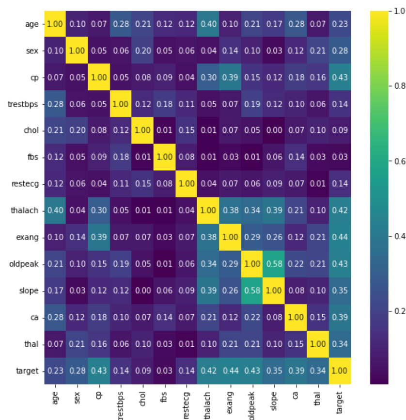
Figure 4. Dataset features heatmap.
