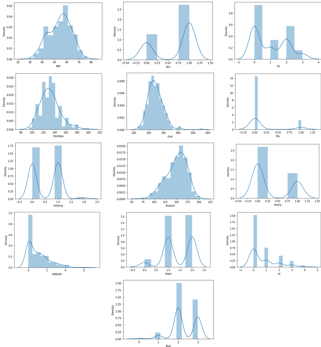
Figure 3. Statistical description of heart disease dataset.
