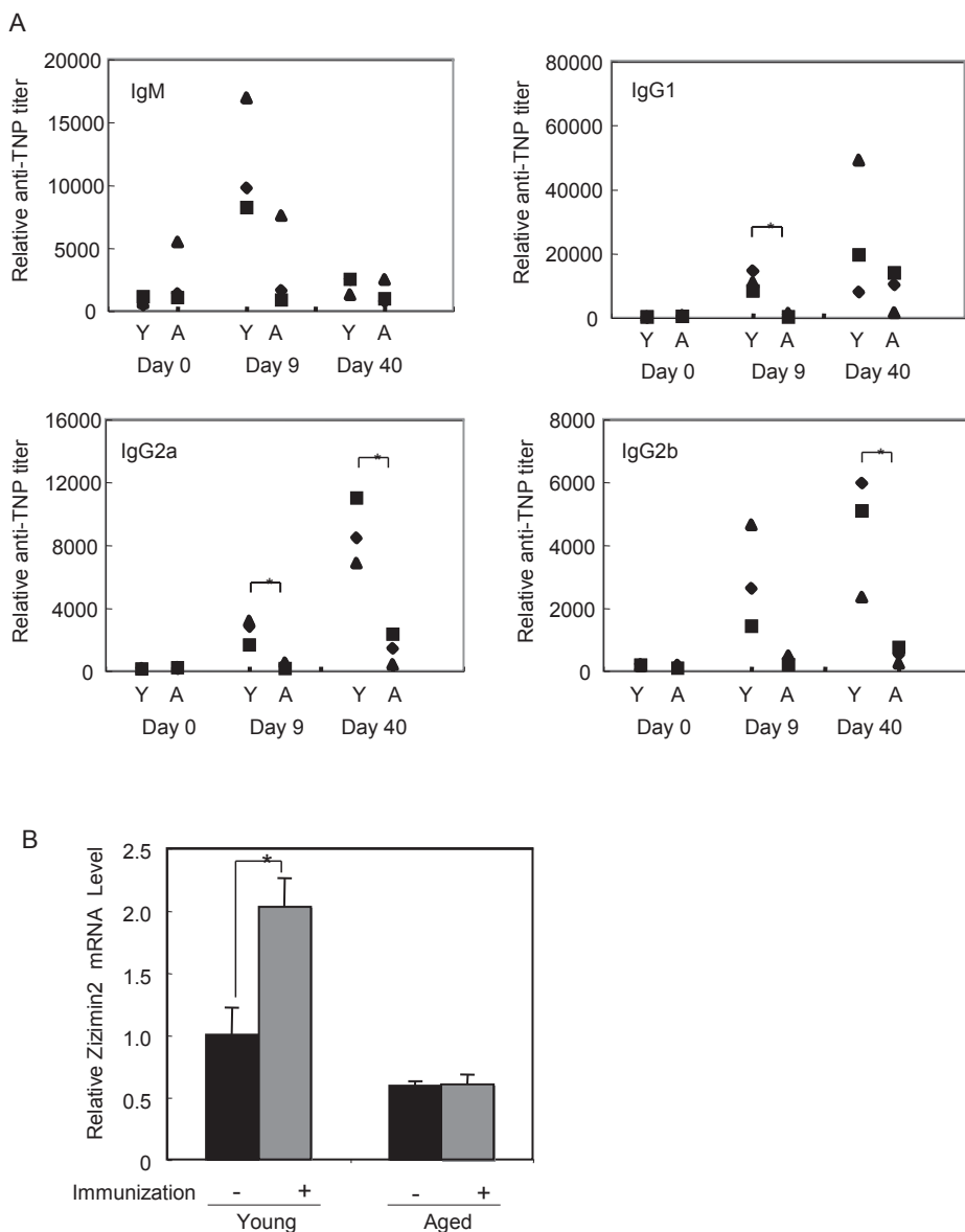
Fig. 3 Immuno-response in young and aged mice.
