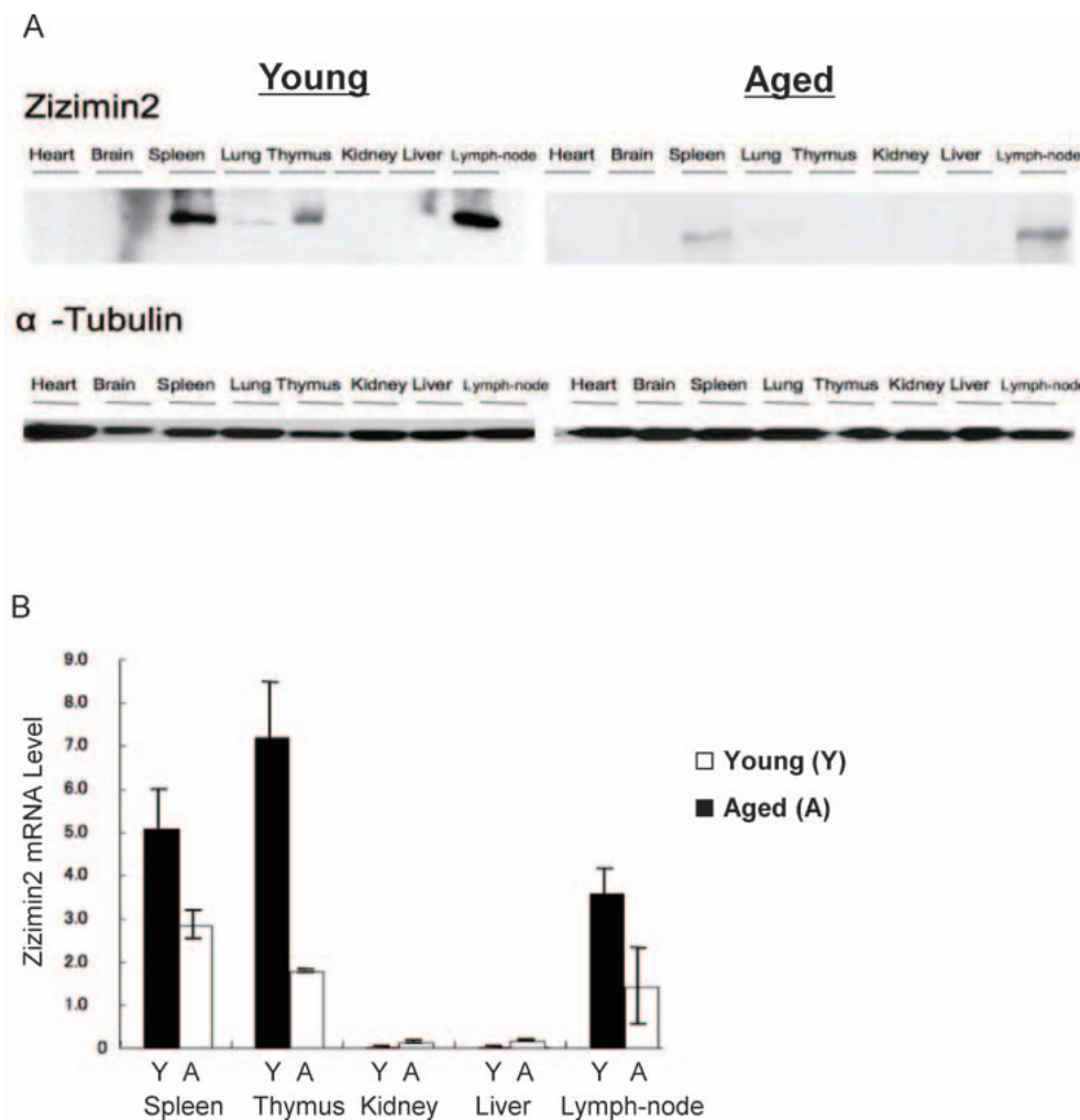
Fig. 2 Expression of Zizimin2 in young and aged mouse. A. Expression of Zizimin2 protein in young and aged mouse. Lysates from the tissues indicated in this figure were prepared. After protein concentration was quantified, an equal amount of protein was subjected to immunoblot analysis. \alpha -Tubulin was used as a loading control. B. Expression of Zizimin2 mRNA in young and aged mice. cDNA from the tissues designated in this figure was subjected to quantitative real-time PCR using gene specific primer set for Zizimin2 or GAPDH. Relative expression levels were calculated by delta-delta CT method using GAPDH as a internal control gene. These results are representative of at least three independent experiments.
