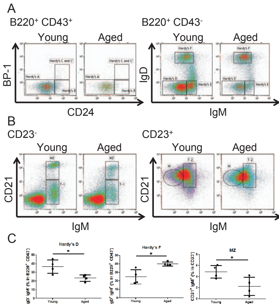
Fig. 1 Flow cytometric analysis of B cell development in bone marrow and spleen.
