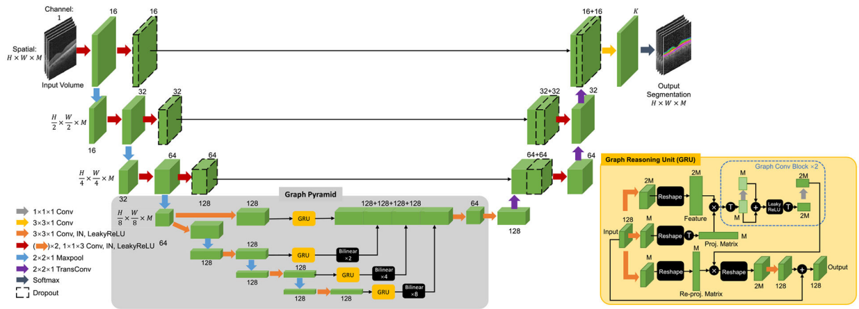
FIGURE 4. Proposed 3D OCT segmentation network with graph pyramid architecture. Here “IN” operation denotes Instance Normalization, “LReLU” denotes LeakyReLU activation, “ \otimes ” in black circle denotes transpose, and “ \times ” in black circle denotes matrix multiplication.
