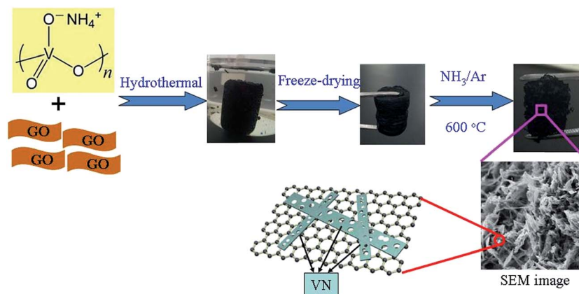
Fig. 1 Schematic diagram for preparing the 3D PVNN/RGO composite.
