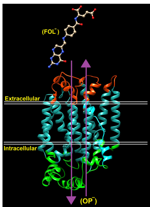
Fig. 4. Overview of folate transporter (RFC (reduced folate carrier/SLC19A1), organic phosphate [OP - ]).
