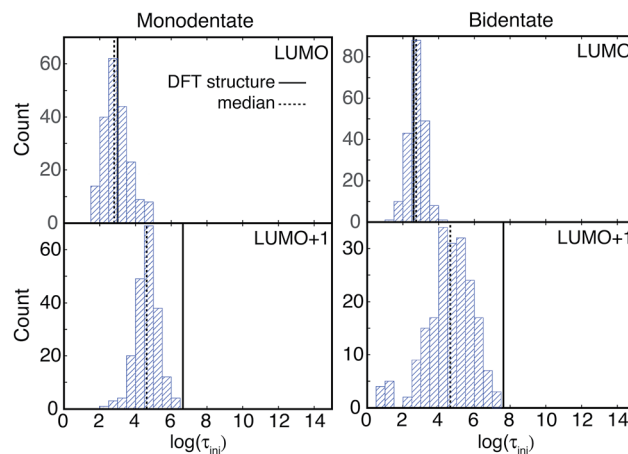
Fig. 10 Distribution of \tau_{\text{ini}} values (log scale) for injection from the LUMO and LUMO+1 initial states of the two attachment modes. The \tau_{\text{ini}} values for the DFT-optimized structures are indicated by solid lines, and the median \tau values for the sampled structures are shown as dashed lines.
