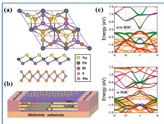
Fig. 8 (a) Top and side view of the crystal structure of the NaPbBi/MoS 2 heterostructure, with the supercell of 2 × 2 NaPbBi on the 3 × 3 MoS 2 substrate, which matches well. (b) Schematic model of NaPbBi/MoS 2 HTS for quantum state measurement. Vertical arrows show the spin orientation of electrons in the edge states and horizontal arrows show their transport directions. (c) The band structure without and with SOC in which the red, green, and blue dots represent p_{xy} , p_z , and s states, respectively, while yellow dots represent the MoS 2 substrate effect.
