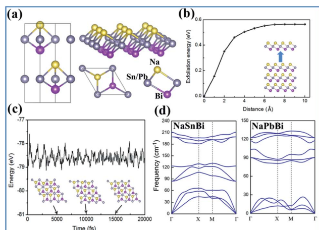
Fig. 1 (a) Top view and side view of 2D NaXBi (X = Sn/Pb), (b) cleavage energy of NaSnBi, (c) snapshots of atomic configurations of NaSnBi at the end of MD simulations at 5, 10 and 15 ps at a temperature of 300 K, respectively. (d) Calculated phonon spectrum dispersions of mono-layers NaSnBi (left) and NaPbBi (right).
