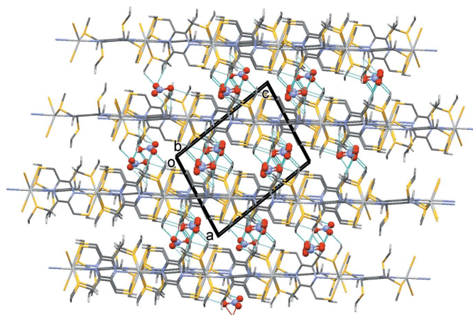
Figure 5 A view along the b axis of compound (I), with emphasis on the crystal packing. Hydrogen bonds are shown as dashed lines (see Table 4), and only those H atoms involved in intermolecular C—H \cdots O hydrogen bonds have been included.
