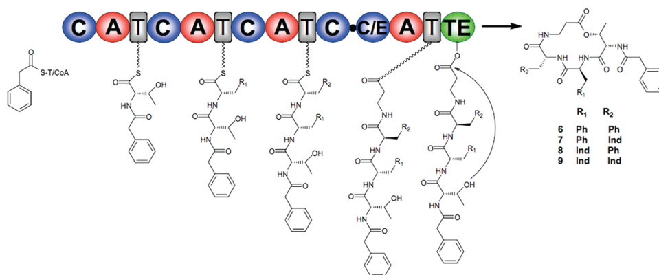
Figure 2. Proposed xenematide biosynthesis. Xenematide A (9) and several new xenematide derivatives B (6), C (7), and D (8) are shown. Compound 4 is the open chain methanolysis product of xenematide A, which is not shown. Ph, phenyl; Ind, indole.
