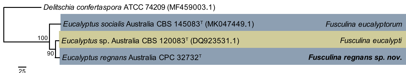
Fig. 40. The single most parsimonious tree obtained from a phylogenetic analysis of the Fusculina ITS sequence alignment (four strains including the outgroup; 690 characters analysed: 393 constant, 284 variable and parsimony-uninformative and 13 parsimony-informative). The tree was rooted to Delitschia confertasporea (GenBank MF459003.1) and the scale bar indicates the number of changes. Bootstrap support values higher than 49 % are shown at the nodes and novelties are highlighted with bold text. Species names are indicated to the right of the tree and GenBank accession numbers between round parentheses. A superscript T denotes strains with a type status. Tree statistics: TL = 339 steps, CI = 0.985, RI = 0.615, RC = 0.606. The analysis was performed using PAUP v. 4.0b10 (Swofford 2003).
