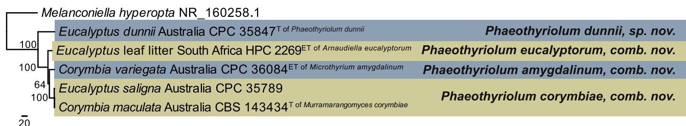
Fig. 81. The single most parsimonious trees obtained from a phylogenetic analysis of the Phaeothyriolum ITS sequence alignment (six strains including the outgroup; 585 characters analysed: 297 constant, 238 variable and parsimony-uninformative and 50 parsimony-informative). The tree was rooted to Melanconiella hyperopta (GenBank NR_160258.1) and the scale bar indicates the number of changes. Bootstrap support values higher than 49 % are shown at the nodes and novelties are highlighted with bold text. Species names are indicated to the right of the tree. A superscript T denotes strains with a type status and ET those with ex-epitype status. Tree statistics: TL = 364 steps, CI = 0.962, RI = 0.745, RC = 0.717. The analysis was performed using PAUP v. 4.0b10 (Swofford 2003).
