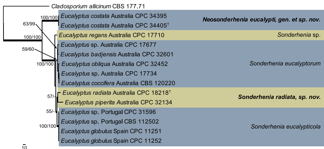
Fig. 101. The first of 11 equally most parsimonious trees obtained from a phylogenetic analysis of the Sonderhenia combined ITS, act , cmdA and tub2 sequence alignment (15 strains including the outgroup; 1686 characters analysed: 1254 constant, 325 variable and parsimony-uninformative and 107 parsimony-informative). The tree was rooted to Cladosporium allacinum (GenBank DQ780399.1, EF679489.1, EF679565.1, EF101451.1, respectively) and the scale bar indicates the number of changes. Thickened branches represent those present in the strict consensus parsimony tree. Bootstrap support values higher than 49 % are shown at the nodes (parsimony bootstrap support / NJ HKY85 distance bootstrap support) and novelties are highlighted with bold text. Species names are indicated to the right of the tree. A superscript T denotes strains with a type status. Tree statistics: TL = 508 steps, CI = 0.951, RI = 0.872, RC = 0.830. The analyses were performed using PAUP v. 4.0b10 (Swofford 2003).
