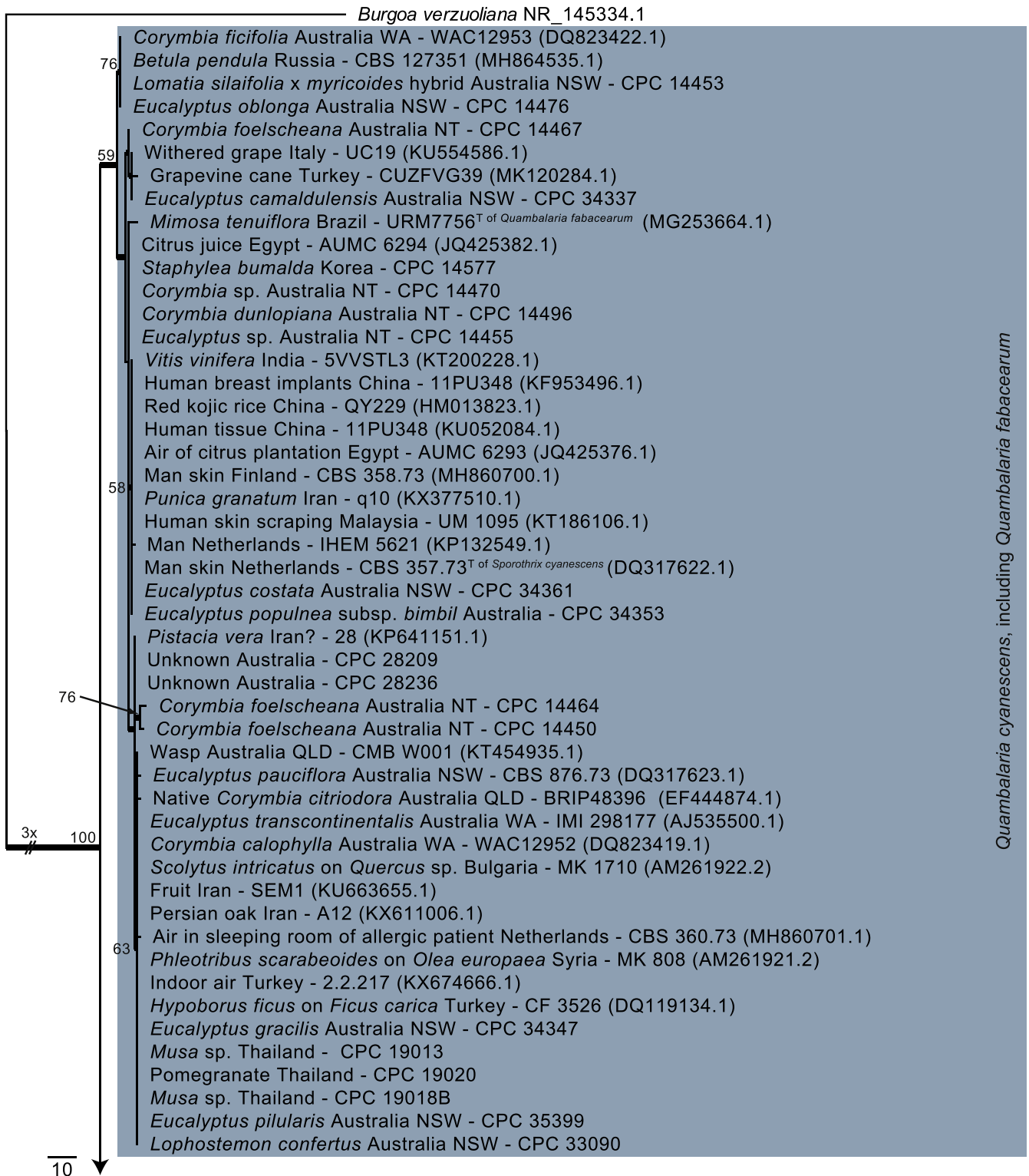
Fig. 95. The first of 384 equally most parsimonious trees obtained from a phylogenetic analysis of the Quambalaria ITS sequence alignment (105 strains including the outgroup; 581 characters analysed: 317 constant, 189 variable and parsimony-uninformative and 75 parsimony-informative). The tree was rooted to Burgoa verzuoliana (GenBank NR_145334.1) and the scale bar indicates the number of changes. Thickened branches represent those present in the strict consensus parsimony tree. Bootstrap support values higher than 49 % are shown at the nodes and novelties are highlighted with bold text. Species names are indicated to the right of the tree and GenBank accession numbers between round parentheses. A superscript T denotes strains with a type status and ET those with ex-epitype status. Tree statistics: TL = 364 steps, CI = 0.860, RI = 0.973, RC = 0.837. The analysis was performed using PAUP v. 4.0b10 (Swofford 2003).
