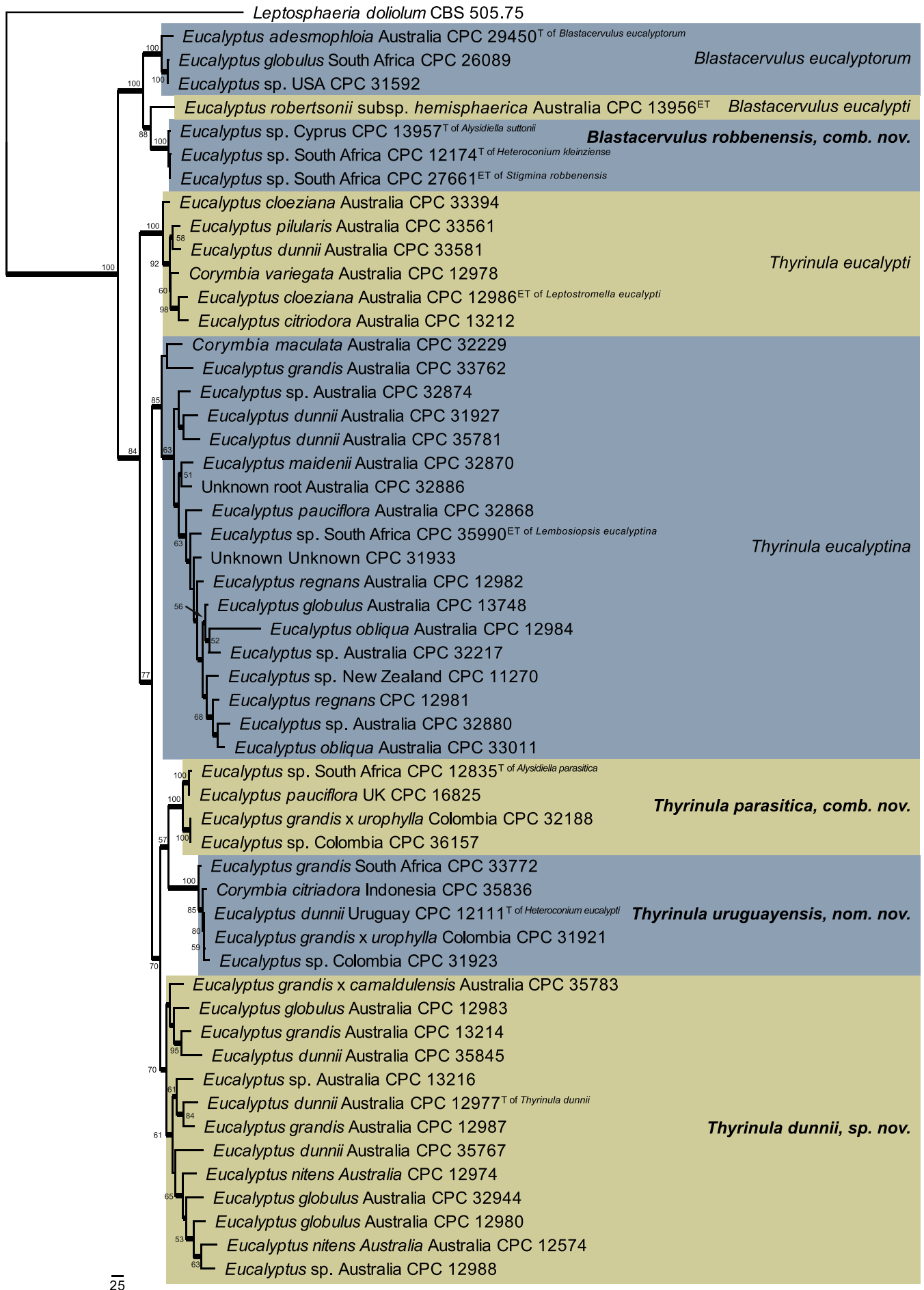
Fig. 12. The first of 45 equally most parsimonious trees obtained from a phylogenetic analysis of the Blastacervulus/Thyrinula combined ITS, LSU, chs , second part of tef1 and tub2 sequence alignment (54 strains including the outgroup; 2919 characters analysed: 1881 constant, 542 variable and parsimony-uninformative and 496 parsimony-
