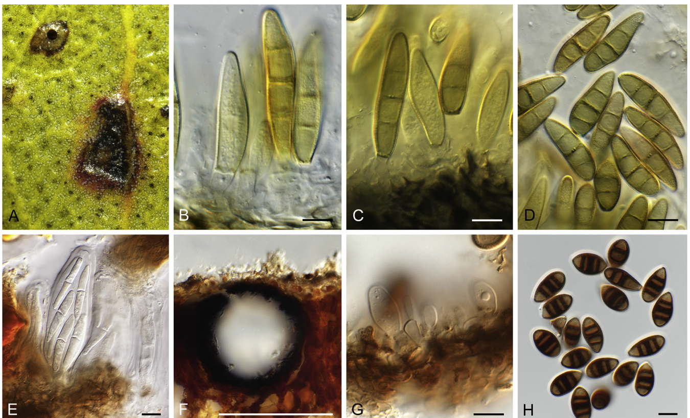
Fig. 57. Neosonderhenia spp. A–D. N. eucalypti (CBS 145081). A. Leaf spot. B–D. Conidiogenous cells and conidia. E–H. N. foliorum [K(M) 251545]. E. Ascus with ascospores. F. Transverse section through conidioma. G. Conidiogenous cells. H. Conidia. Scale bars: F = 250 \mu m, all others = 10 \mu m.
