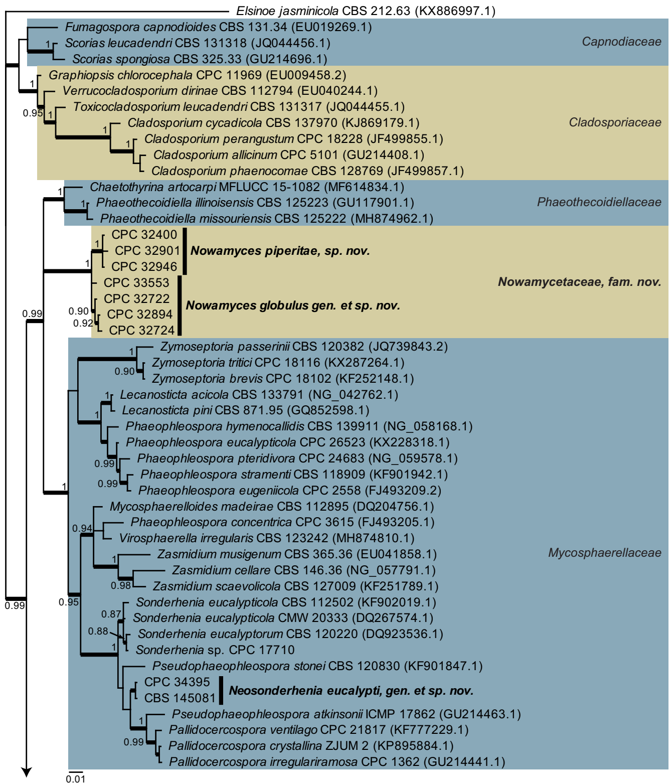
Fig. 61. Consensus phylogram (50 % majority rule) of 182 252 trees resulting from a Bayesian analysis of the Capnodiales LSU sequence alignment (90 strains including the outgroup; 779 aligned positions; 258 unique site patterns). The tree was rooted to Elsinoe jasminicola (GenBank KX886997.1) and the scale bar indicates the expected changes per site. Bayesian posterior probabilities (PP) >0.84 are shown at the nodes and novelties are highlighted with bold text. Family names are indicated to the right of the tree and GenBank accession numbers between round parentheses. Thickened branches represent those present in the strict consensus parsimony tree. The analyses were performed using MrBayes v. 3.2.6 (Ronquist et al. 2012) and PAUP v. 4.0b10 (Swofford 2003). The parsimony analysis (only strict consensus branches showed) yielded the maximum of 1 000 equally most parsimonious trees and had the following statistics: 529 constant, 59 variable and parsimony-uninformative and 193 parsimony-informative characters; TL = 890 steps, CI = 0.415, RI = 0.842, RC = 0.349.
