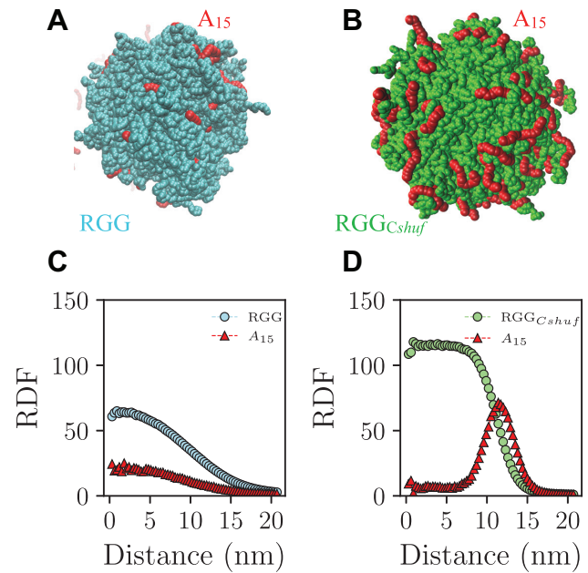
Figure 5. Protein sequence dependent protein-polynucleotide phase separation persists in a droplet simulation: (A) Snapshot of the A 15 /LAF-1 RGG condensate and (B) snapshot of the A 15 /LAF-1 RGG Cshuf condensate. Radial distribution functions (RDF) from droplet simulations also show a well-mixed condensate for the (C) A 15 /LAF-1 RGG mixture and interfacial peaks for the (D) A 15 /LAF-1 RGG Cshuf mixture at 220K.
