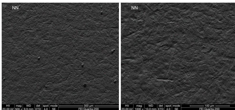
Figure 5 SEM image of the sandblasting group with no porcelain sintering. SEM, scanning electron microscopy; NN, no porcelain sintering and agent.
