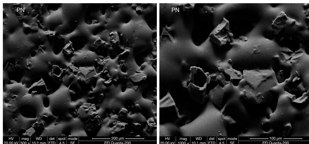
Figure 8 SEM image of the control group with porcelain sintering. SEM, scanning electron microscopy; PN, porcelain sintering + no agent.
