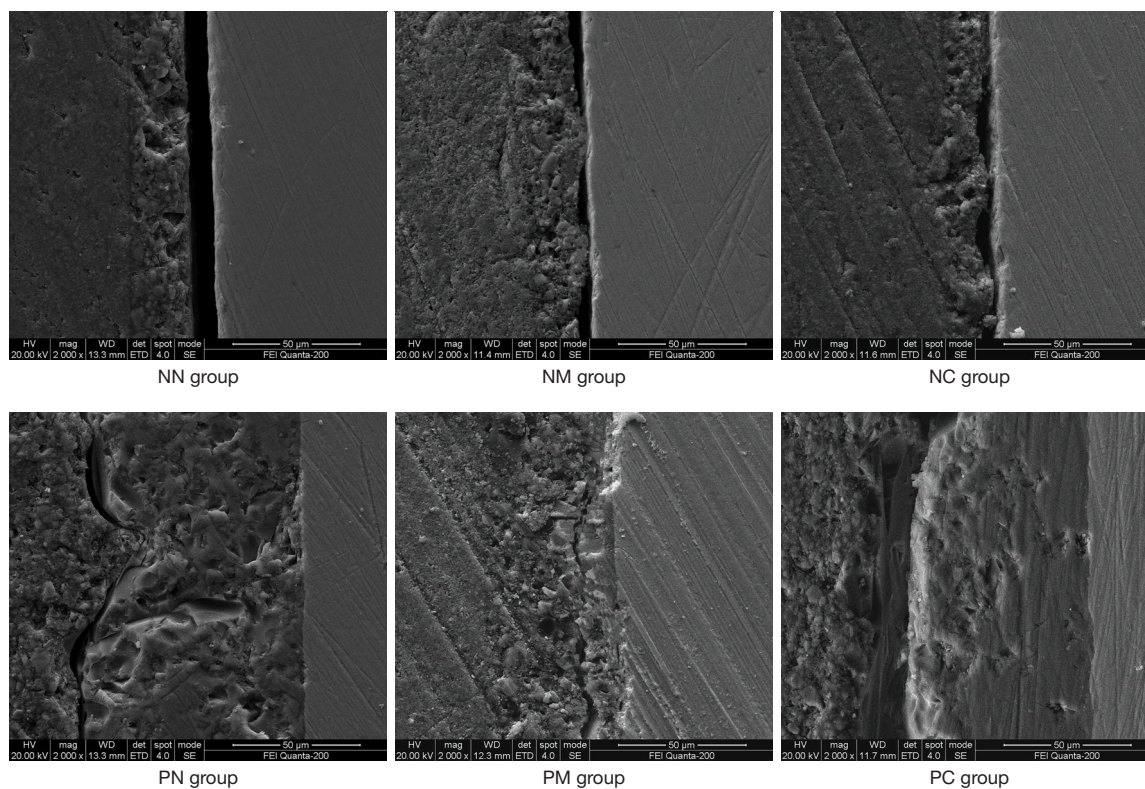
Figure 13 SEM scan graphs of the bonding interfaces of specimens in each group . SEM, scanning electron microscopy; NN, no porcelain sintering and agent; NM, no porcelain sintering + Monobond-S; NC, no porcelain sintering + Clearfil Repair; PN, porcelain sintering + no agent; PM, porcelain sintering + Monobond-S; PC, porcelain sintering + Clearfil Repair.
