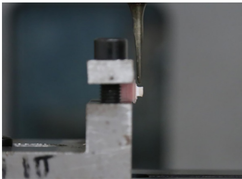
Figure 2 Shear force test.
