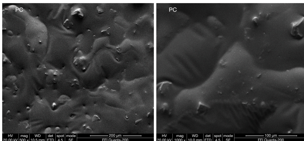
Figure 10 SEM image of the Clearfil Repair treatment group with porcelain sintering. SEM, scanning electron microscopy; PC, porcelain sintering + Clearfil Repair.
