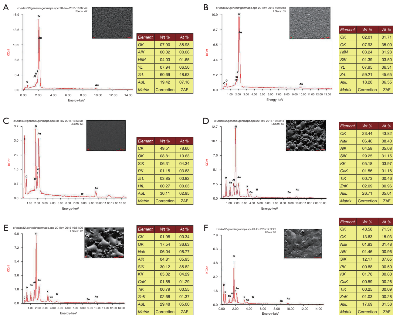
Figure 11 Energy spectrum analysis of the group after surface treatment. (A) NN group; (B) NM group; (C) NC group; (D) PN group; (E) PM group; (F) PC group. NN, no porcelain sintering and agent; NM, no porcelain sintering + Monobond-S; NC, no porcelain sintering + Clearfil Repair; PN, porcelain sintering + no agent; PM, porcelain sintering + Monobond-S; PC, porcelain sintering + Clearfil Repair.
