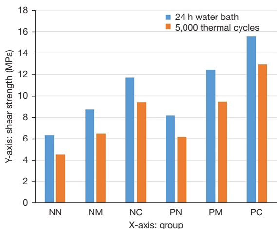
Figure 12 Histogram of the mean shear strength of each experimental group. NN, no porcelain sintering and agent; NM, no porcelain sintering + Monobond-S; NC, no porcelain sintering + Clearfil Repair; PN, porcelain sintering + no agent; PM, porcelain sintering + Monobond-S; PC, porcelain sintering + Clearfil Repair.
