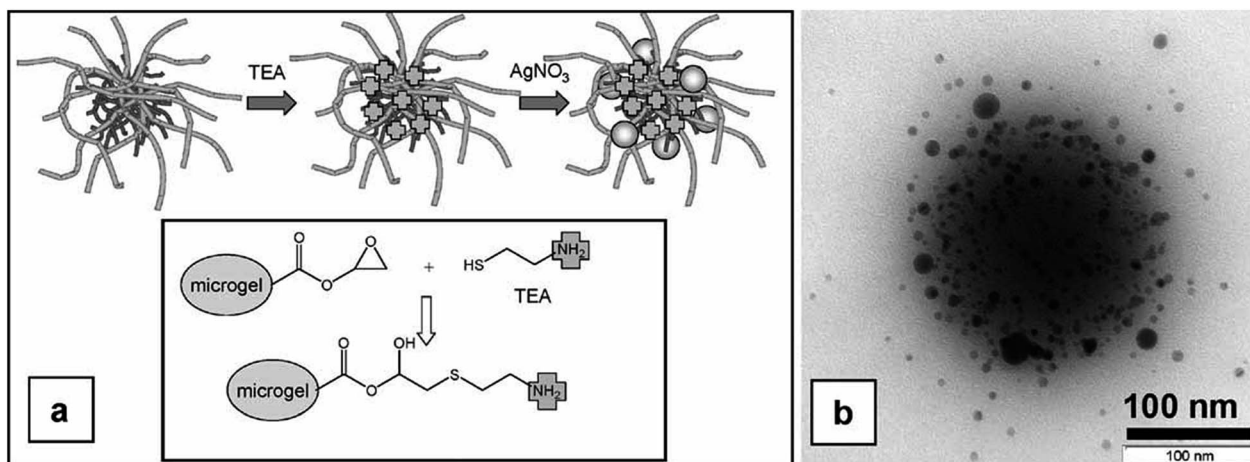
Fig. 3 Modification of poly( N -vinylcaprolactam- co -glycidyl methacrylate) P(VCL-GMA) microgel system with 2-aminoethanethiol (TEA) to obtain modified P(VCL-GMA) microgel particles (a) and TEM image of Ag-P(VCL-GMA) hybrid microgels (b). These images have been reproduced with permission from ref. 48. Copyright©2009 Wiley and Sons.
