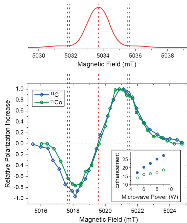
Figure 8. Normalized field-dependent DNP enhancements of 13 C (blue diamonds) and 59 Co (green circles) in 3% Cr(III)-doped [Co(en) 3 Cl 3 ] 2 ·NaCl·6H 2 O measured under 8 W of 140 GHz microwaves with 4 kHz MAS at 80 K. The data were recorded by measuring the spin polarization after constant buildup periods of 50 and 10 s using Bloch decay and Hahn echo sequences for 13 C and 59 Co, respectively. The 140 GHz EPR spectrum (see Figure 2 for details) is shown at the top for comparison. The abscissa is on the same scale but has been shifted because of the slightly different frequencies of the microwave sources used for EPR and DNP. Dashed lines indicate the center of the EPR resonance (red) as well as the respective matching conditions for 13 C (blue) and 59 Co (green). The inset shows the microwave power dependence measured at the field of maximum enhancement.
