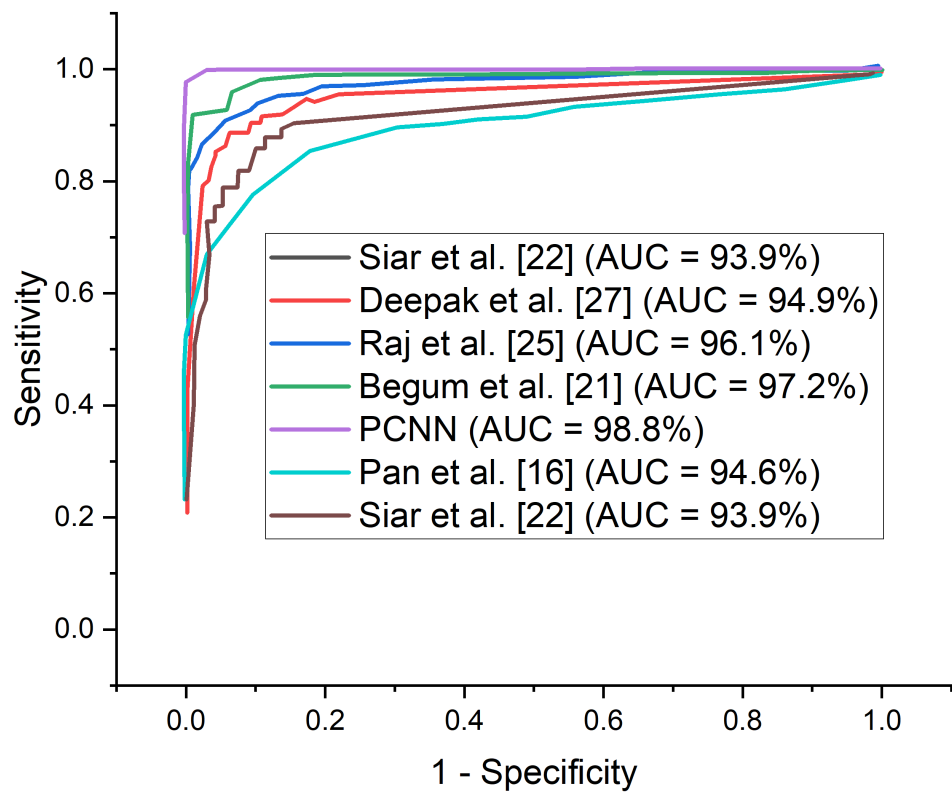
Figure 10. ROC-AUC curves for the proposed PCNN in comparison with some selected state of the art models using the same dataset.
