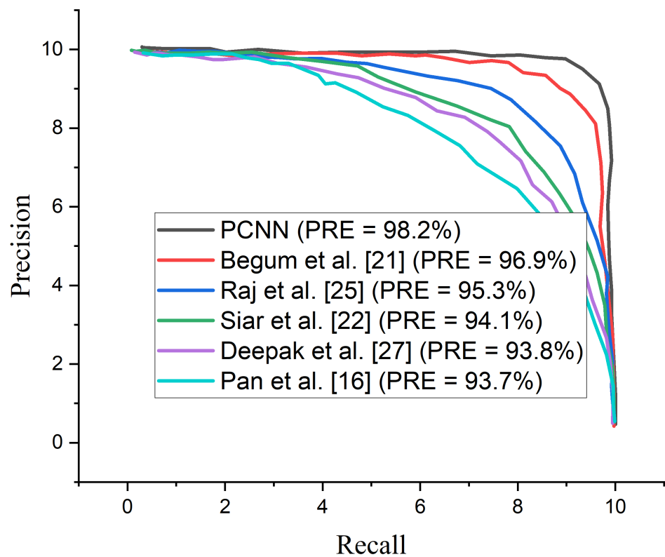
Figure 11. Precision-Recall curves for the proposed PCNN in comparison with some selected state of the art models using the same dataset.
