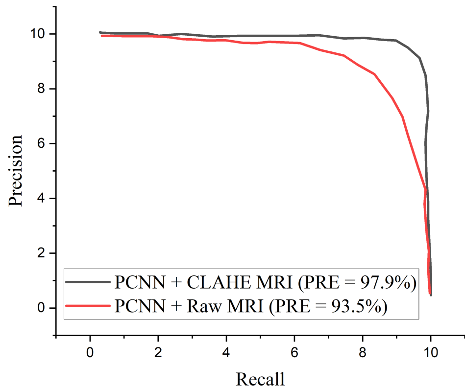
Figure 8. Precision–recall curves for the proposed PCNN in comparison with raw MRI and CLAHE pre-processed MRI images.
