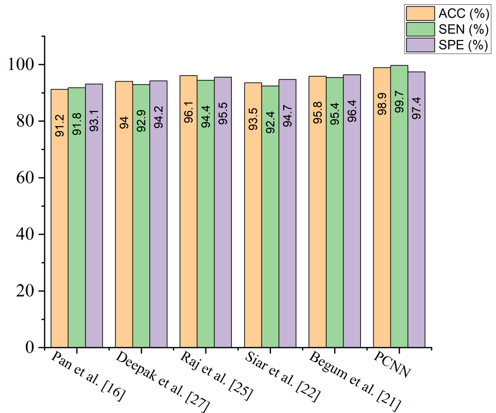
Figure 9. Performance of the proposed PCNN in comparison with some selected state of the art models using the same dataset.
