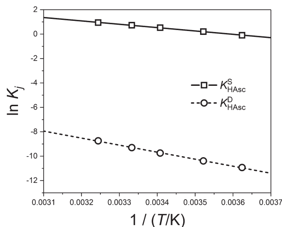
Figure 3. Equilibrium constants K_j in a logarithmic plot over the inverse temperature T . Symbols: calculated from experimental data of this work. Lines: model.
