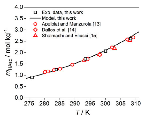
Figure 2. Solubility of vitamin C (HAsc) in molality m in water as a function of the temperature T . Results from this work and data from the literature [13–15].
