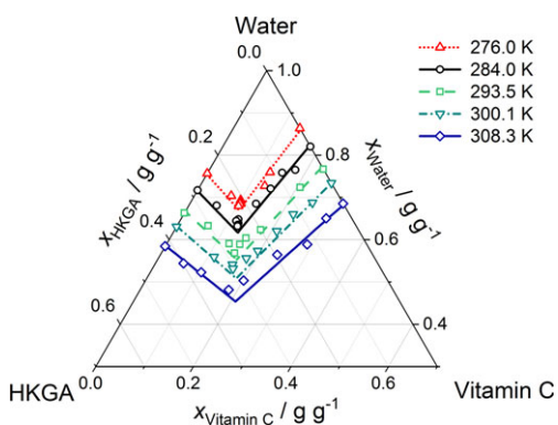
Figure 5. Solid-liquid phase diagram of the system HKGA + vitamin C + water for the studied temperatures at ambient pressure. Symbols: experimental data, this work. Lines: model.
