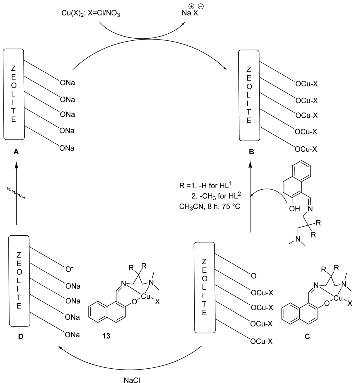
Scheme 12 Synthesis of heterogeneous catalysts via metal (M = Cu) incorporation followed by immobilization of the Schiff base ligands into the zeolite, NaY.
