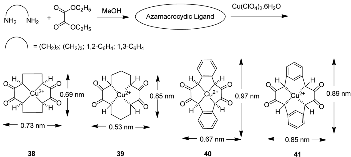
Scheme 38 Synthesis of [\text{Cu}(\text{azamacrocyclic})]^{2+} .
